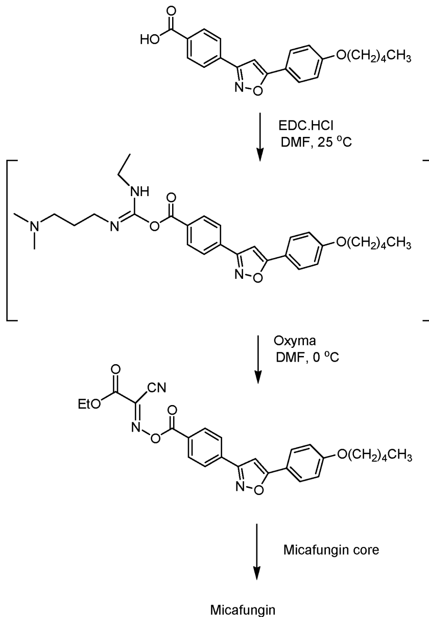
Reaction scheme 1:
