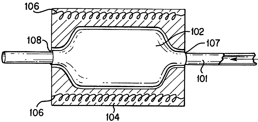
FIG. 15 PRIOR ART
