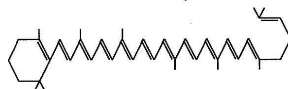
\nu -CAROTENE
