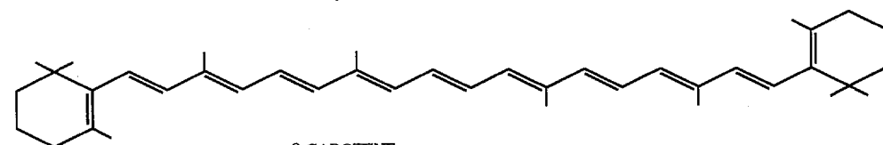
\beta -CAROTENE
