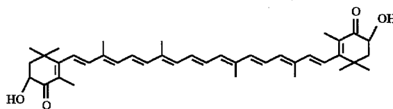
ASTAXANTHIN
