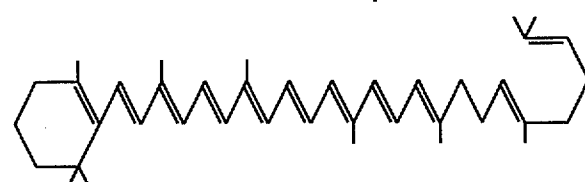
\lambda -ZEACAROTENE
