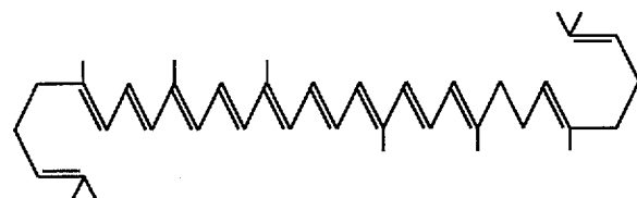
NEUROSPORENE
