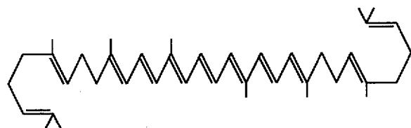
\zeta -CAROTENE
