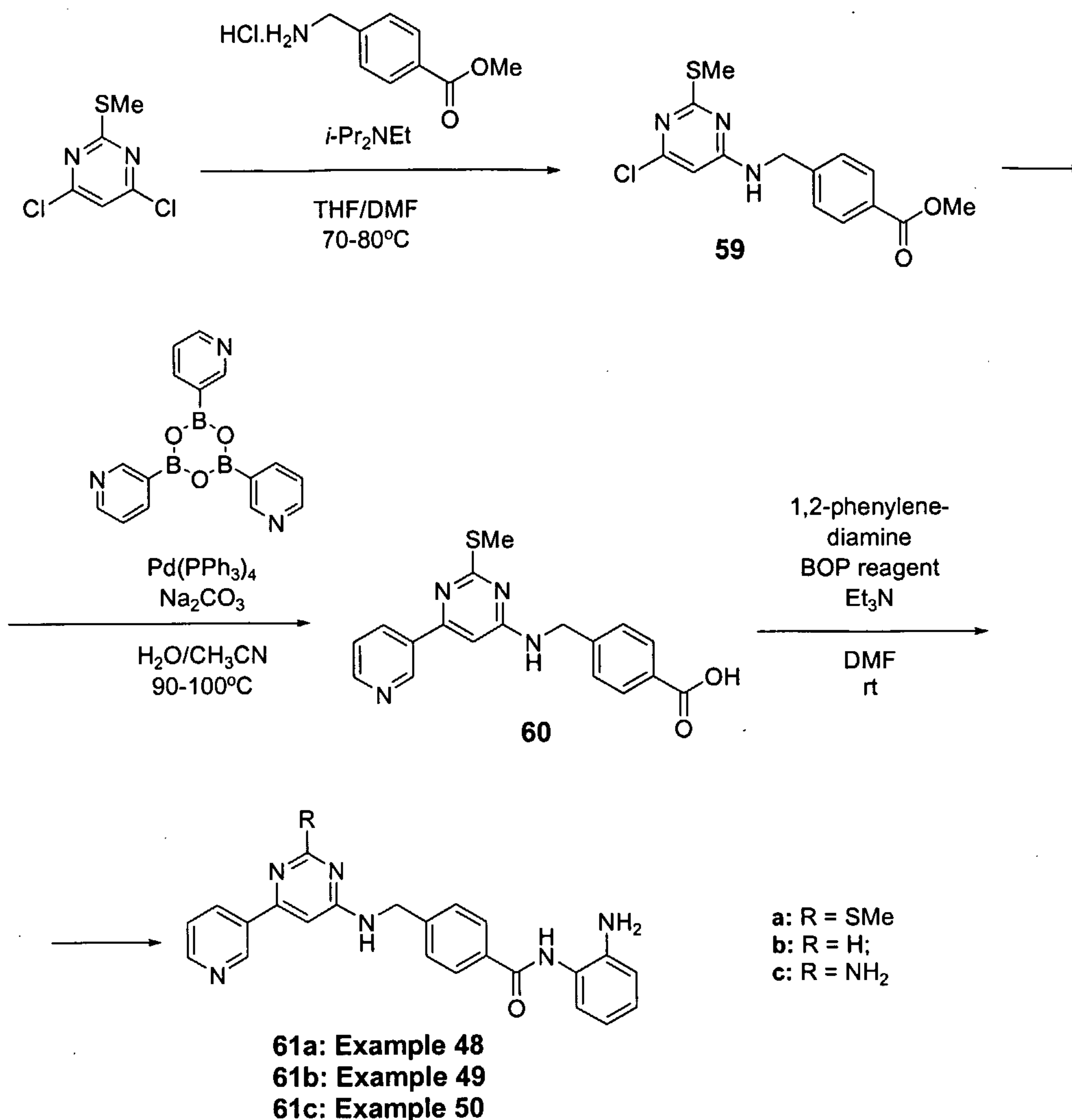
Scheme 16
