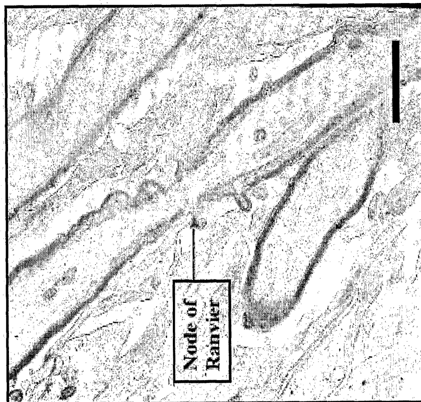
C: LINGO-1-Fc
