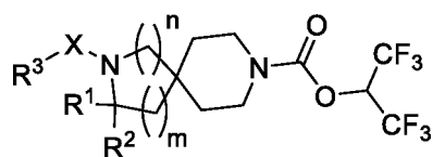
Formula (I);
