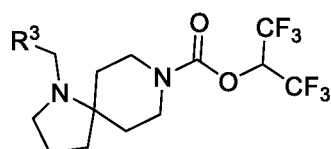
Formula (Ic);
