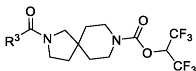
Formula (Ib);
