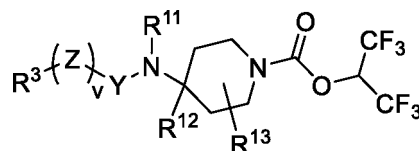
Formula (II);
