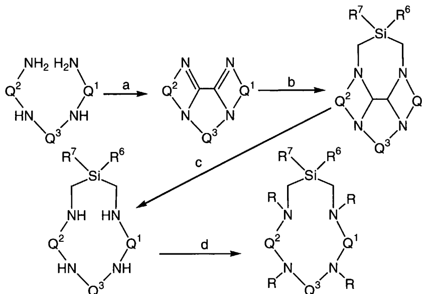
Scheme IX. Synthesis of 1,4,7,10-Tetraaza Macrocyclic Chelants with A Silicone Heteroatom-Bridge.
