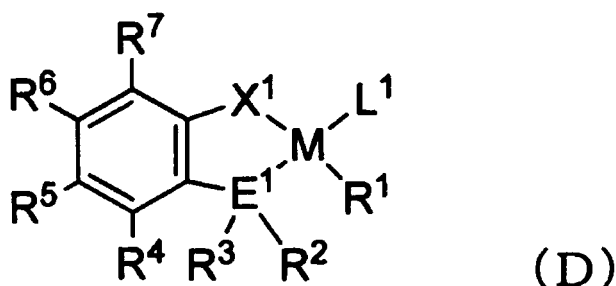
[Chem 2]
