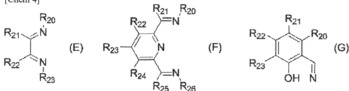
[Chem 4]
