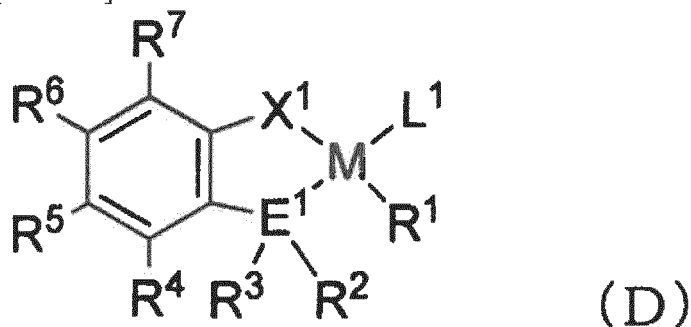
[Chem 2]
