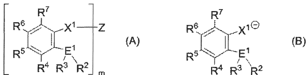
[Chem 4]
