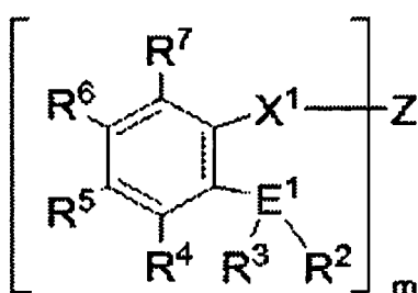
[Chem 1]
