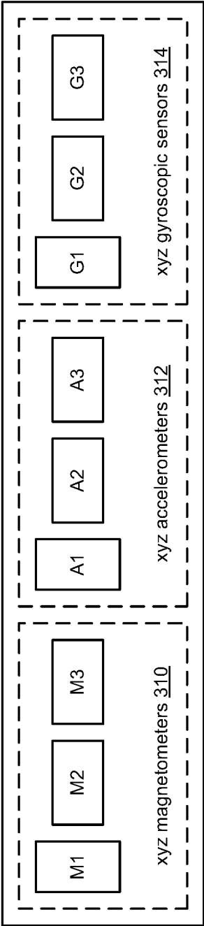
Sensor Instrument Cluster 302 with Three (3) Gyroscopic Sensors 314
