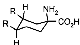
Bucherer-Bergs synthesis
