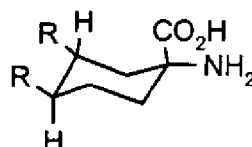
Strecker-synthesis
