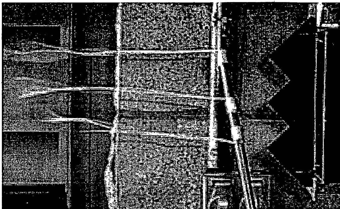
Figure 6. Flow Behind the Sawtooth Tab Mixer
