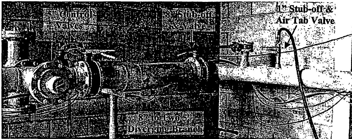
Figure 3. Control Valve Setup
