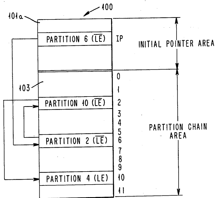
FIG.46 TRANSMIT LIST STRUCTURE IN BURST PRIORITY RAM
