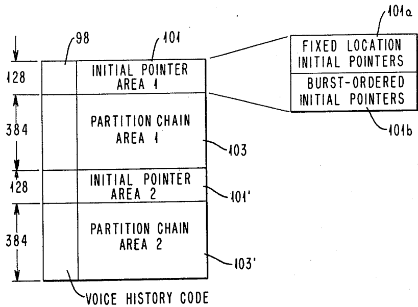
FIG.45 BURST PRIORITY RAM 100
