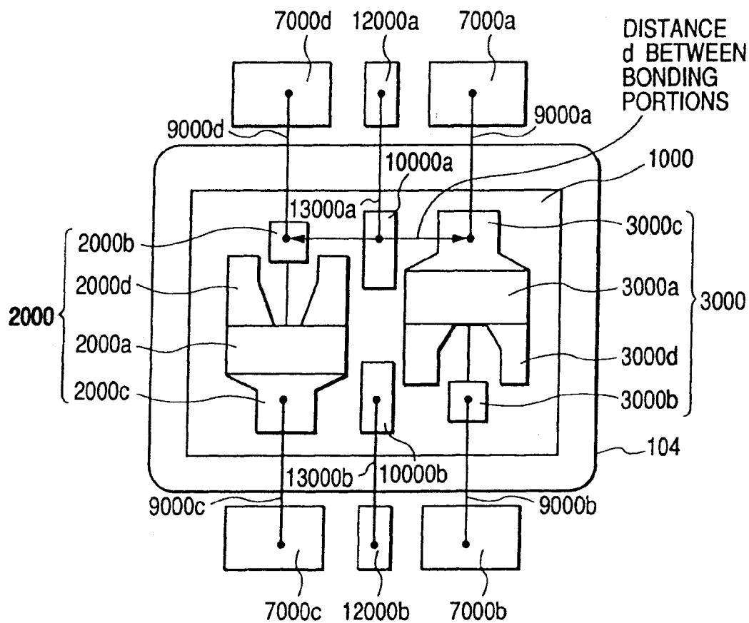
FIG. 21 PRIOR ART
