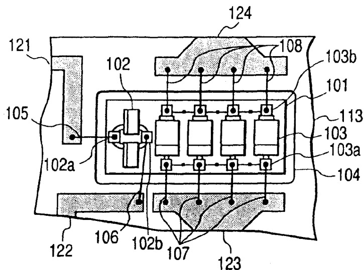
FIG. 21 PRIOR ART
