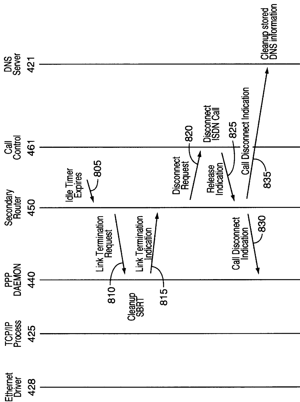
FIG. 8 ISDN CALL DISCONNECT DUE TO IDLE TIMEOUT
