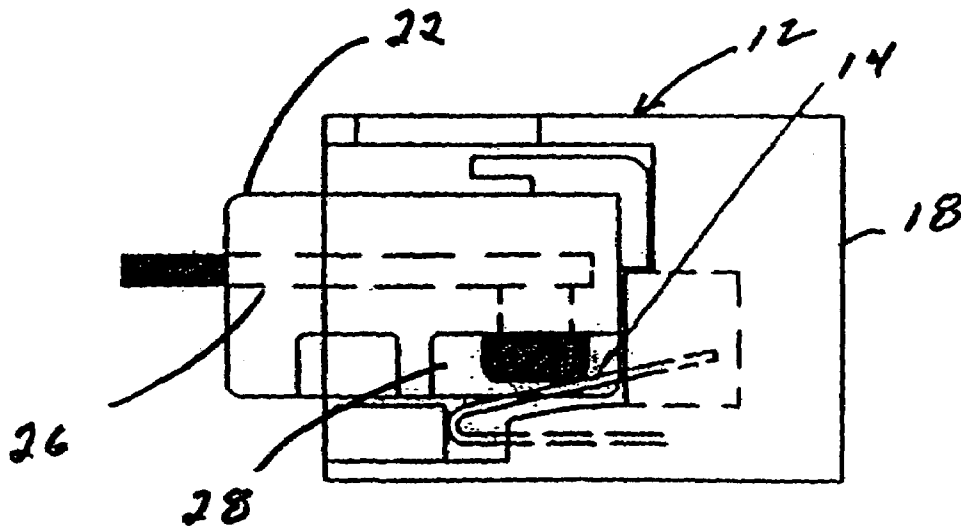
FIG 3 PRIOR ART
