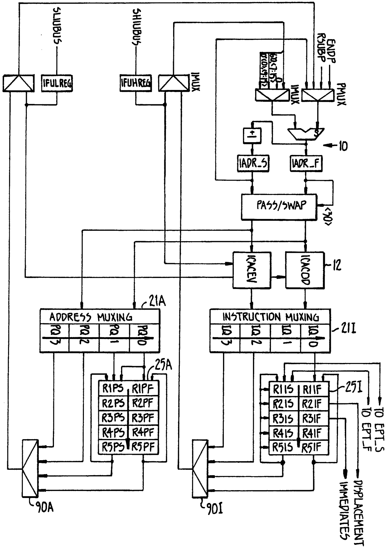
INSTRUCTION CACHE, QUEUE, AND PIPELINE FIG. 11A.
