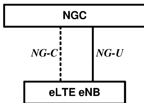
eLTE eNB connected to NGC FIG. 10B
