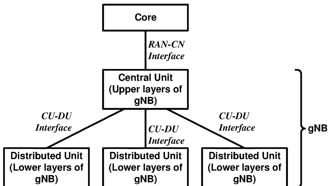
Centralized deployment FIG. 13B
