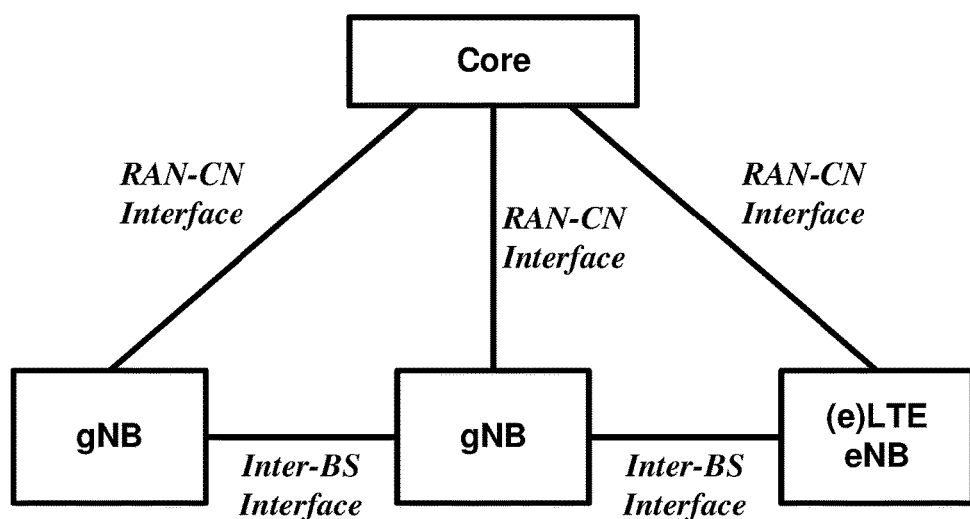
Non-centralized deployment FIG. 13A
