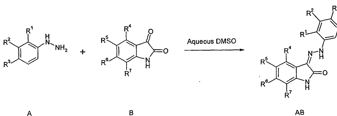
Scheme 2
