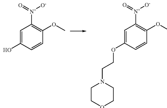
4-[2-(4-Methoxy-3-nitro-phenoxy)ethyl]-morpholine [0285]
