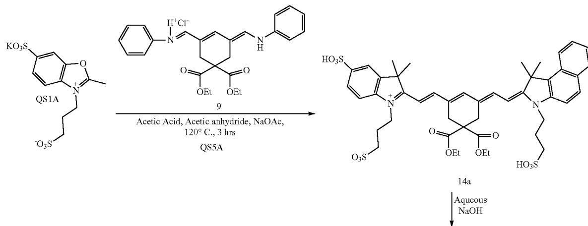
Scheme 3N. Synthesis of Asymmetric Indolinium - Benzindolinium Dye
