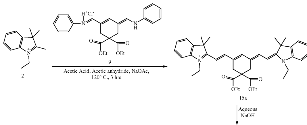
Scheme 3R. Synthesis of Symmetric Indolinium Hydrophobic Dye with two long chain tails
