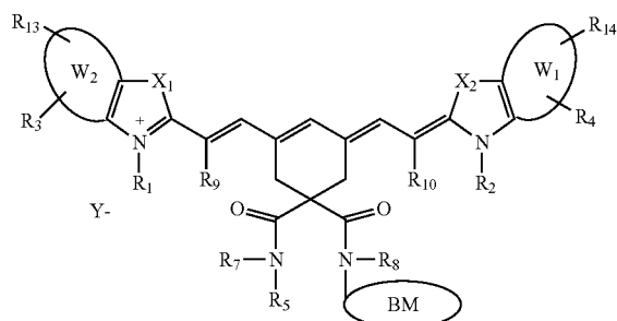
Biomolecule attached fluorophores
