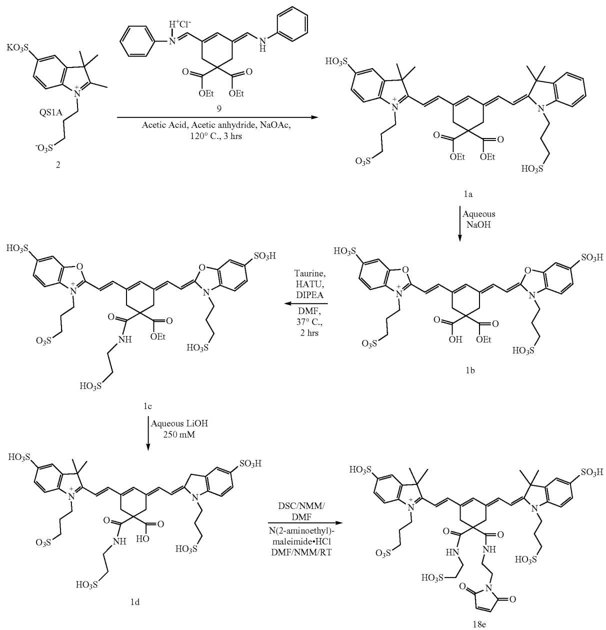
Scheme 3S. Synthesis of Symmetric Indolinium Hydrophilic Maleimide Dye
