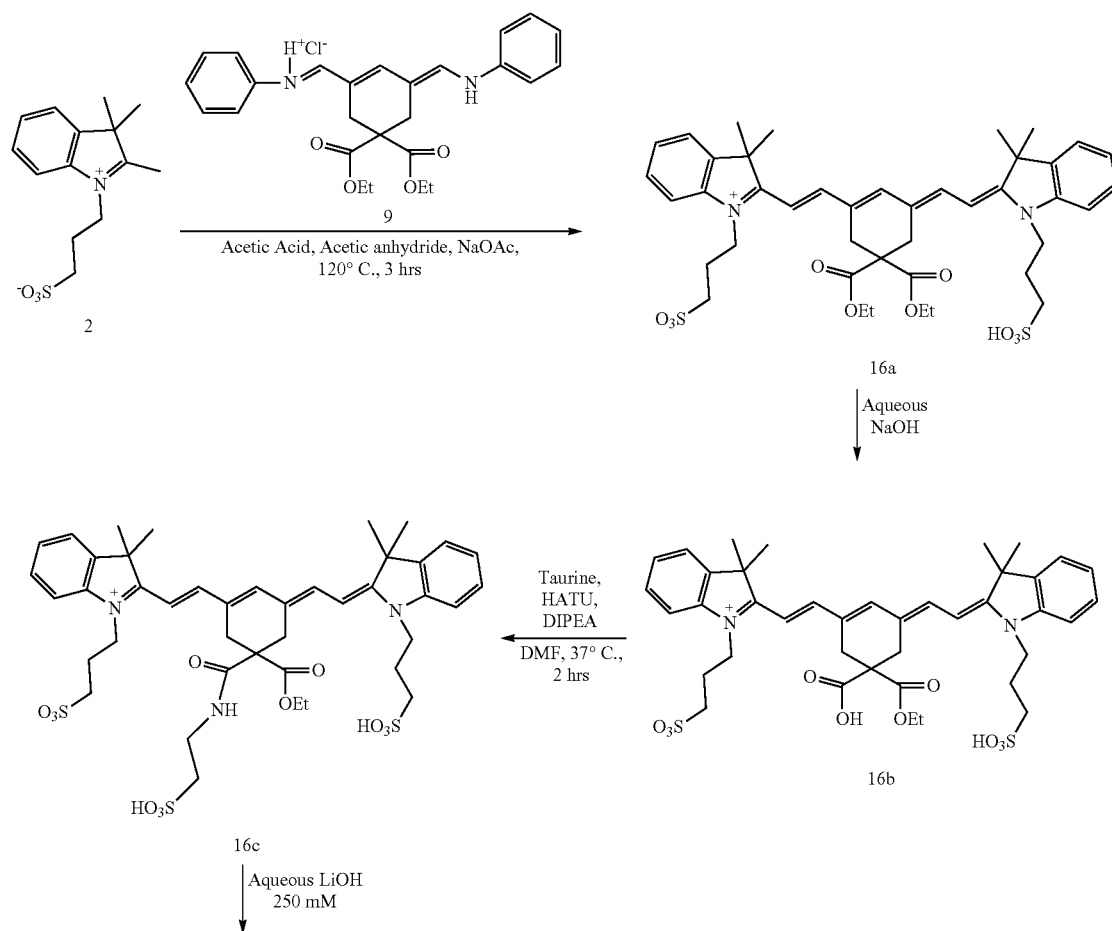
Scheme 3Q. Synthesis of Symmetric Indolinium Dye
