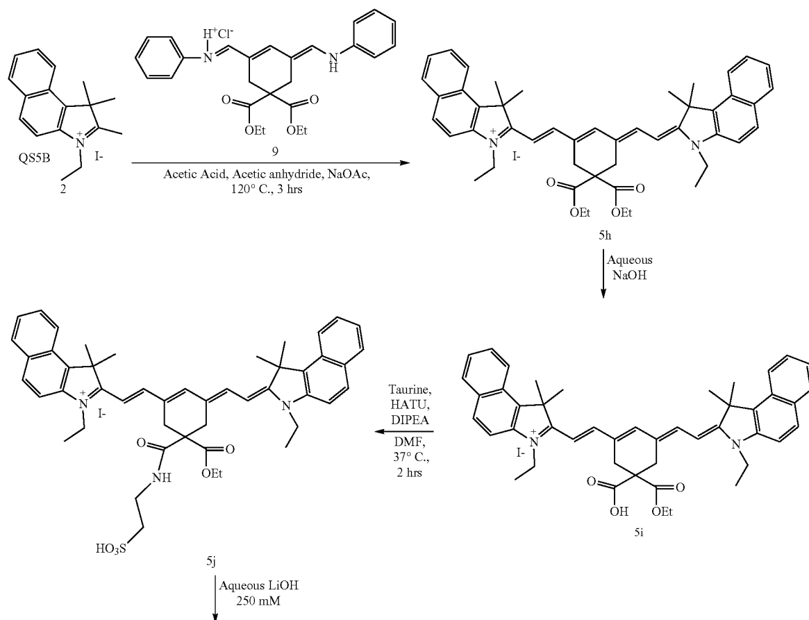
Scheme 3J. Synthesis of Symmetric Benzindole Dye
