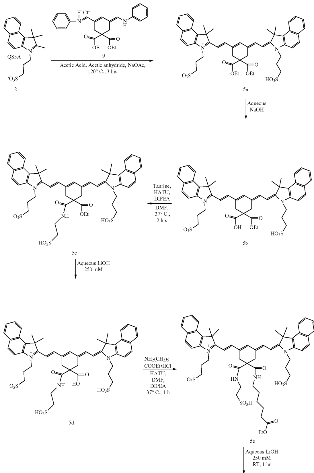
Scheme 3I. Synthesis of Symmetric Benzindole Dye
