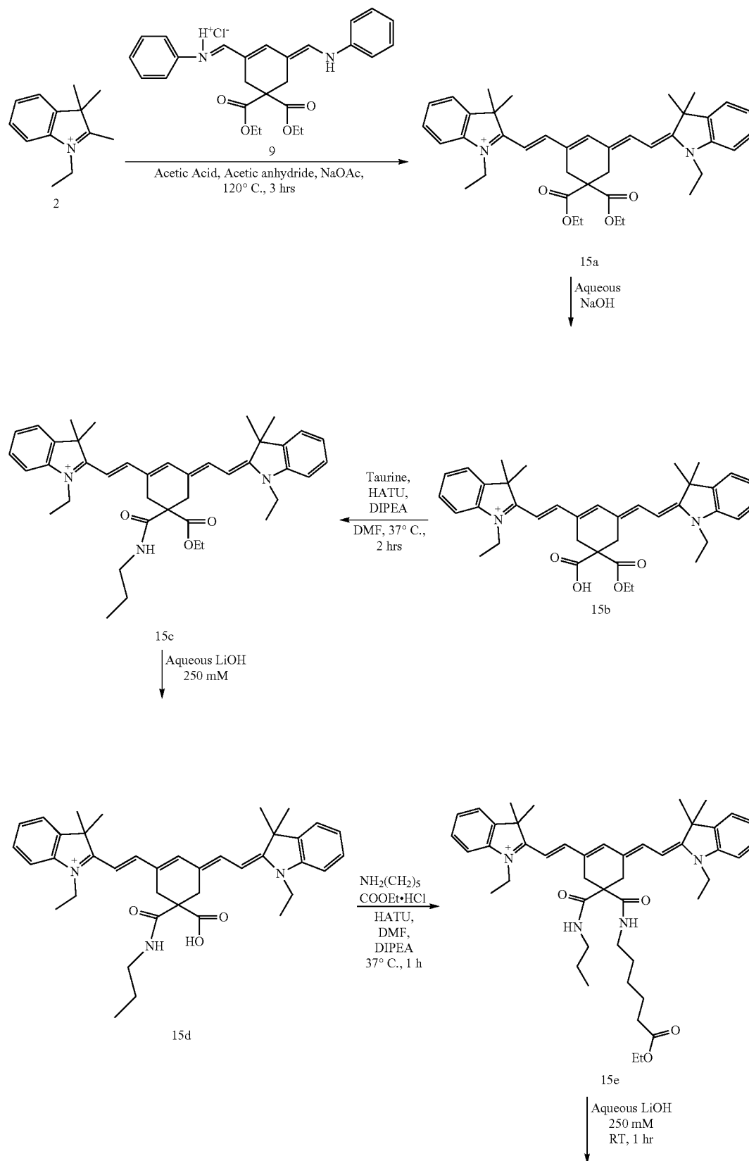
Scheme 3P. Synthesis of Symmetric Indolinium Hydrophobic Dye
