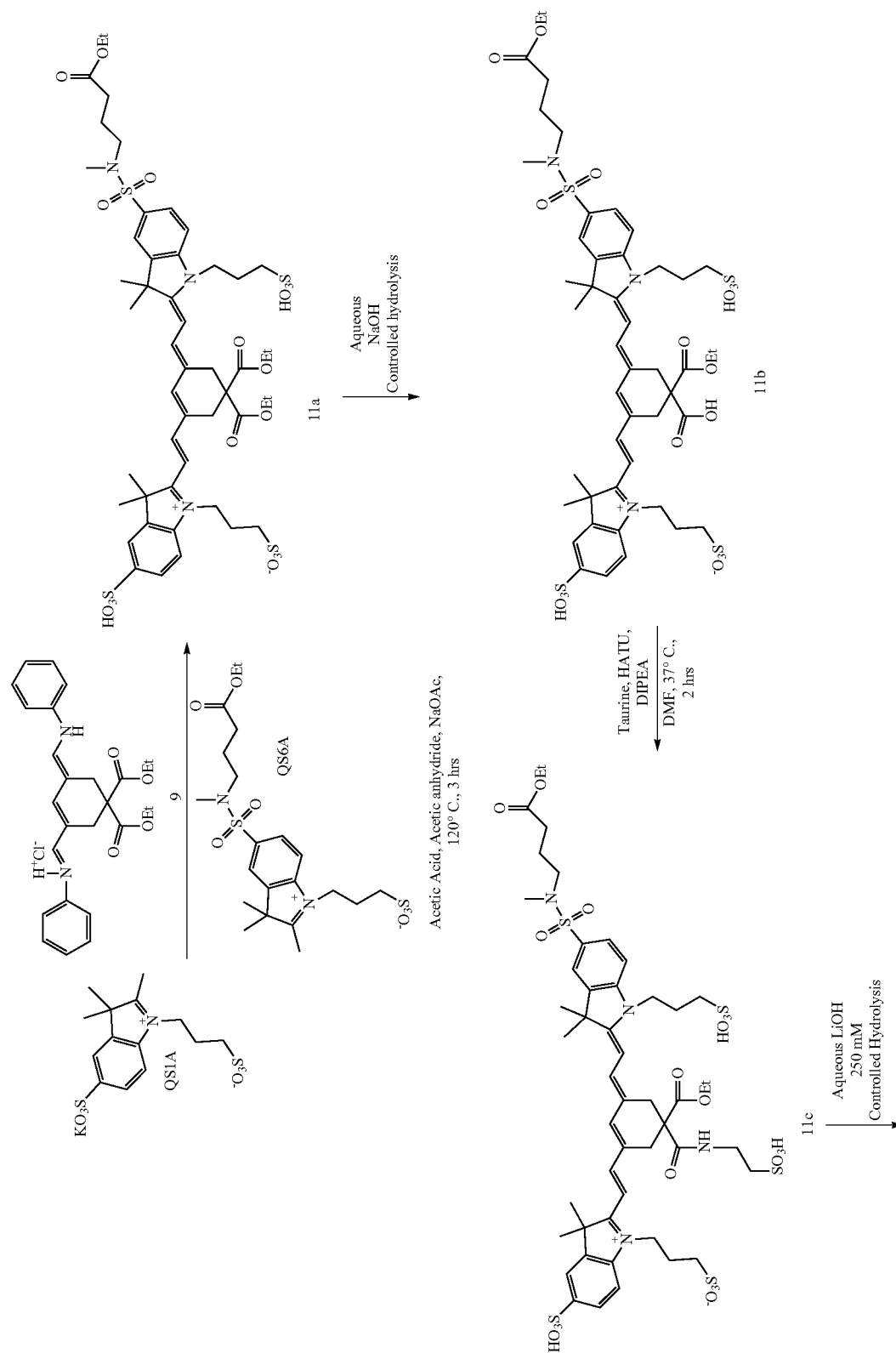
Scheme 3K. Synthesis of Asymmetric Indolinium Dye
