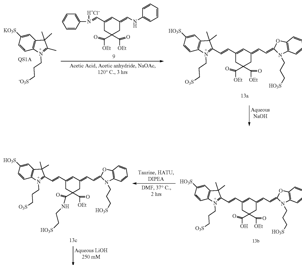
Scheme 3M. Synthesis of Asymmetric Indolinium - Bezoxazole Dye
