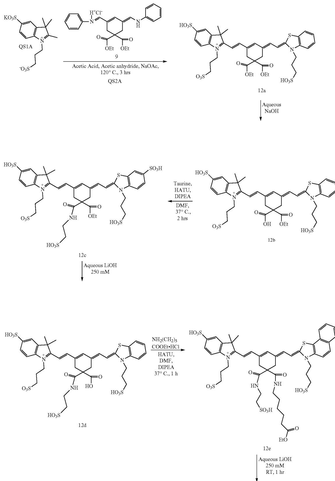
Scheme 3L. Synthesis of Asymmetric Indolinium-Benzothiazole Dye
