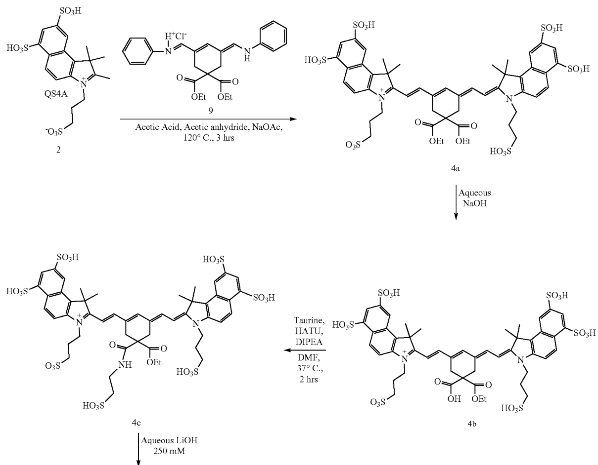
Scheme 3G. Synthesis of Symmetric Benzindole Dye
