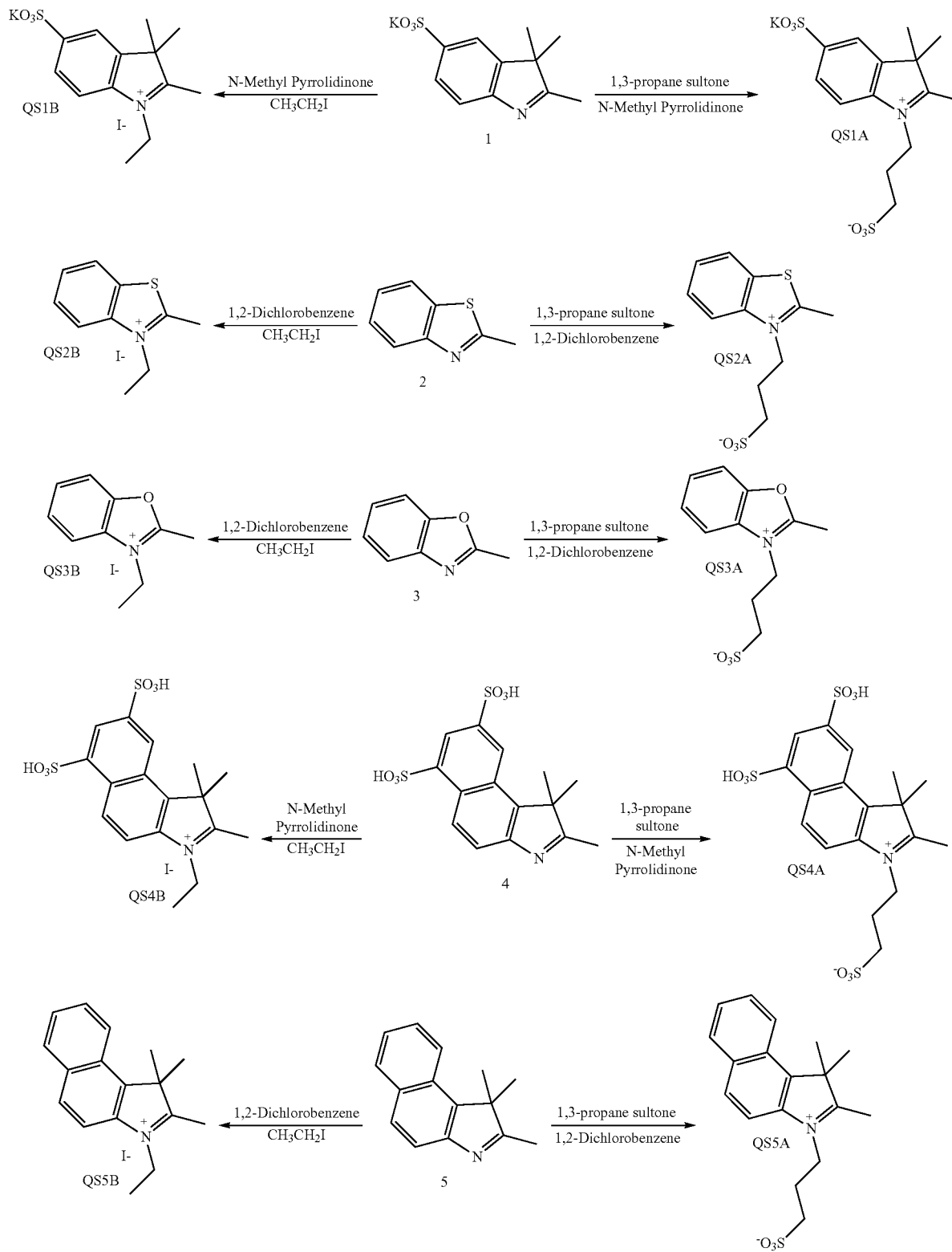
Scheme 1. Preparation of Quaternary Salts
