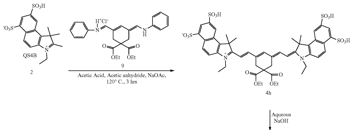
Scheme 3H. Synthesis of Symmetric Benzindole Dye
