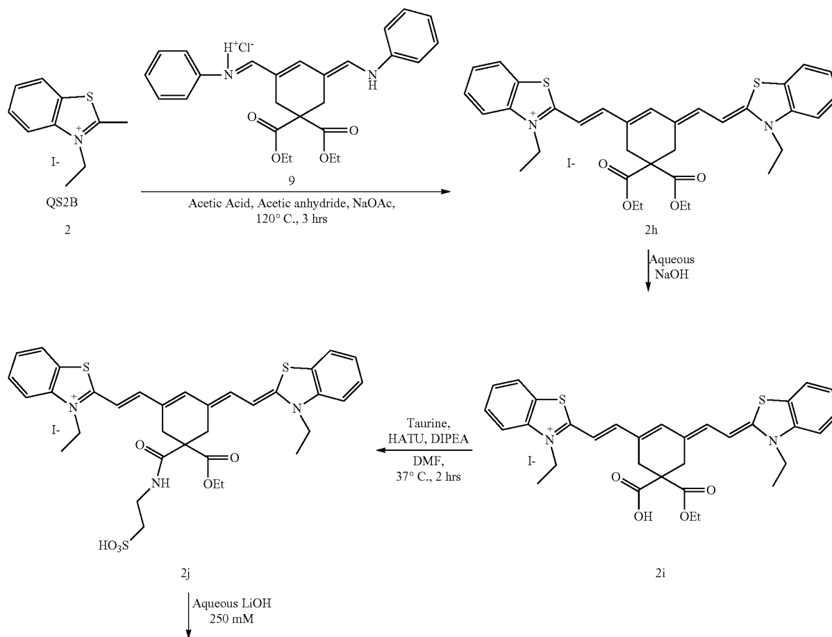
Scheme 3D. Synthesis of Symmetric Benzothiazolium Dye
