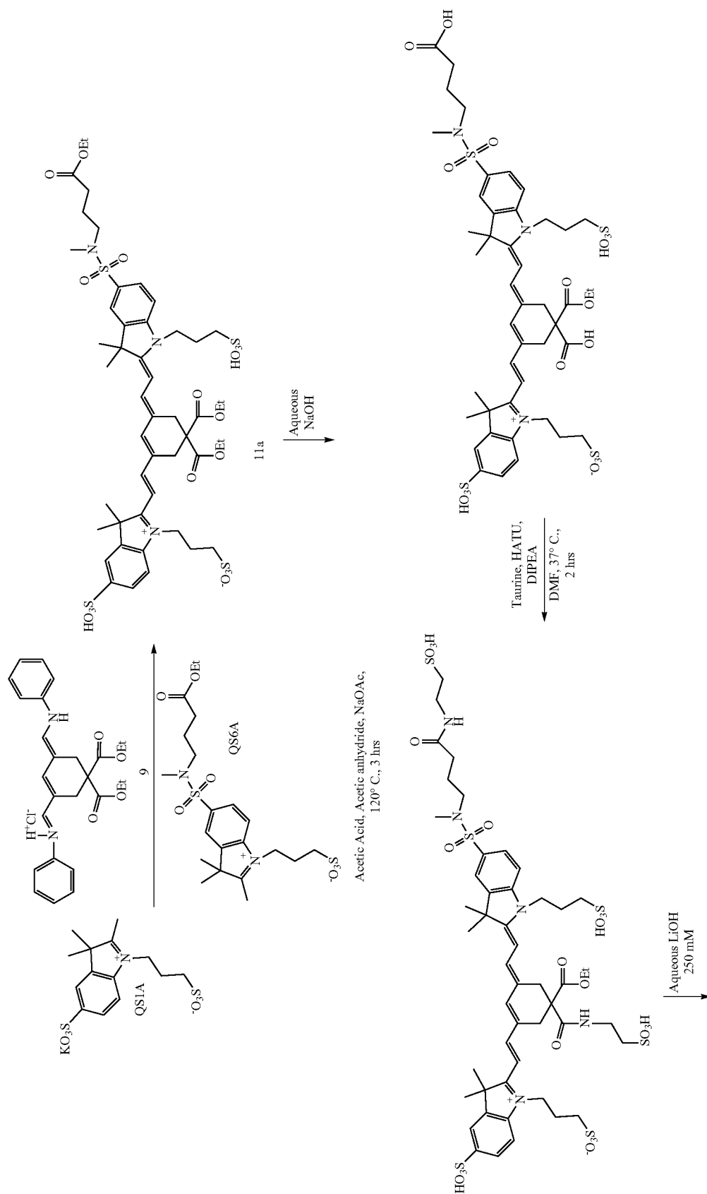
Scheme 3T. Synthesis of Asymmetric Indolinium Dye
