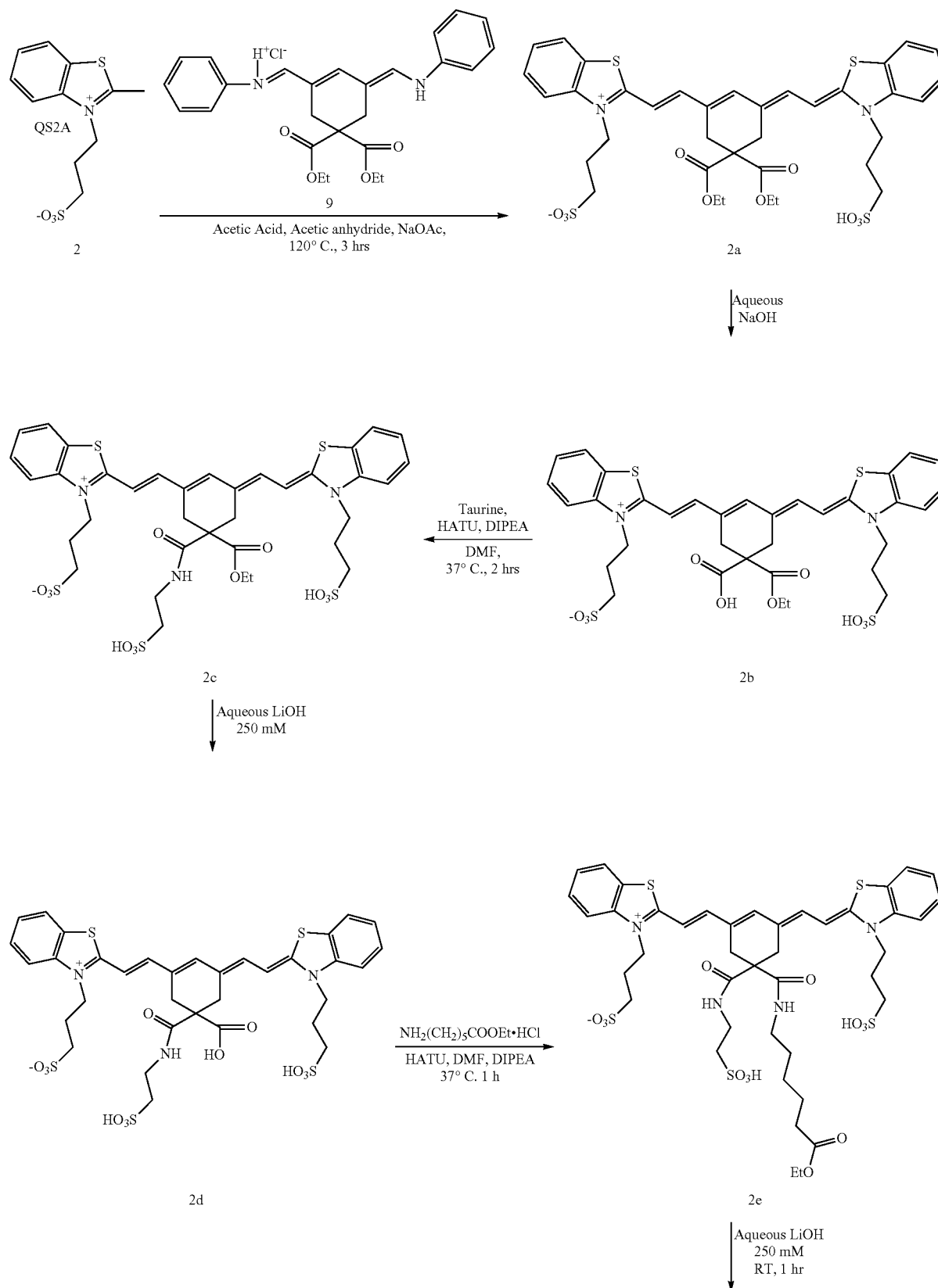
Scheme 3C. Synthesis of Symmetric Benzothiazolium Dye
