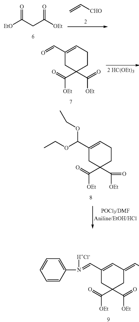
Scheme 2. Preparation of Bridge
