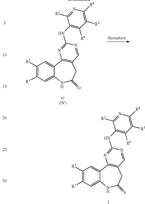
Scheme 1: General route for the synthesis of compounds of formula I
