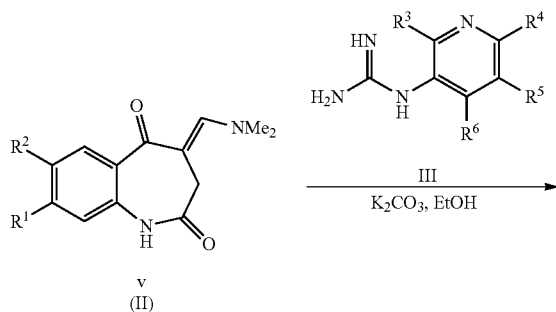
Scheme 2: alternate route for the synthesis of compounds of formula I
