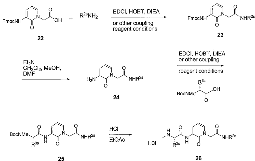
Scheme 7
