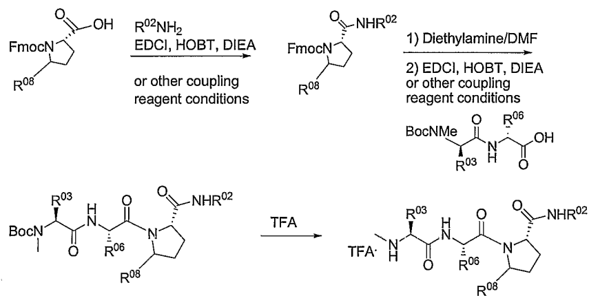
Scheme 19:
