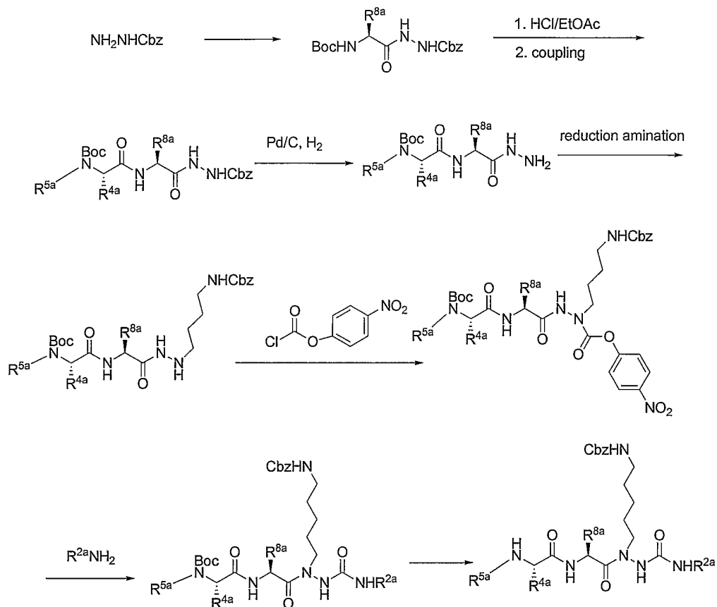
Scheme 26:
