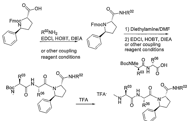
Scheme 18:
