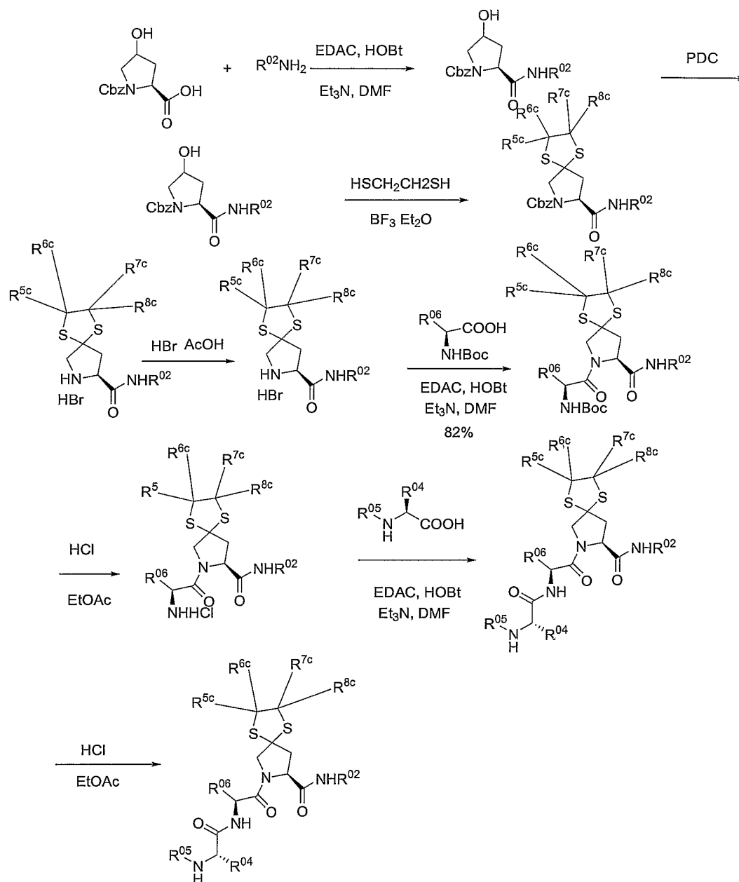
Scheme 27:
