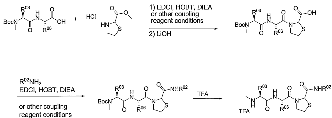
Scheme 16:
