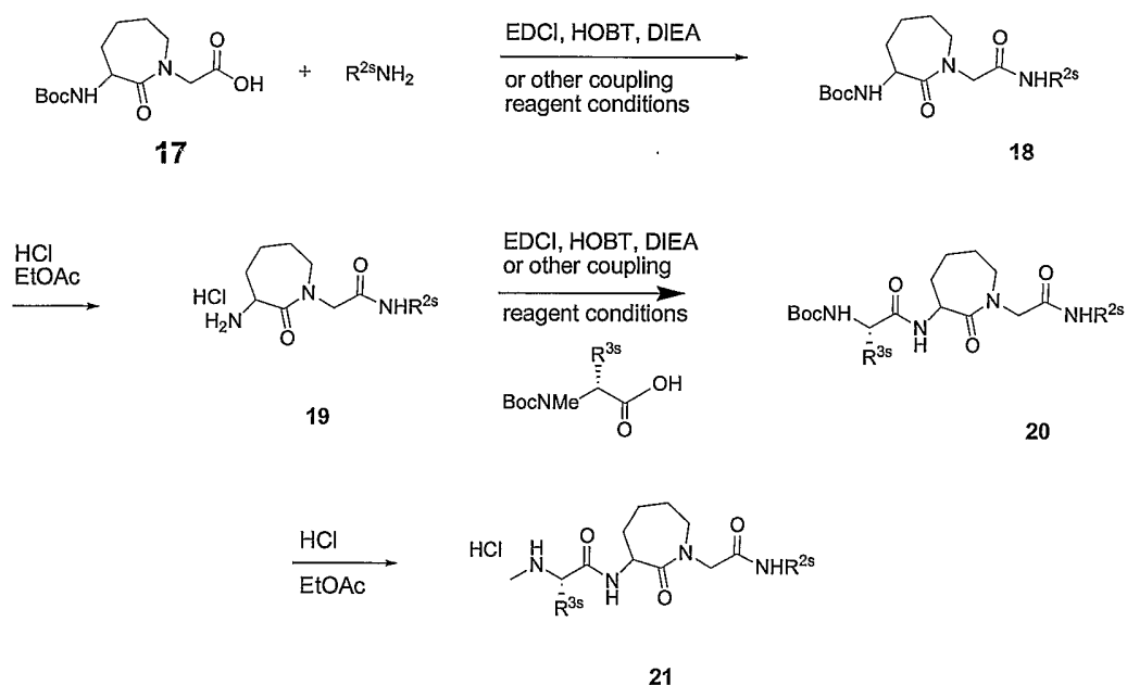
Scheme 6
