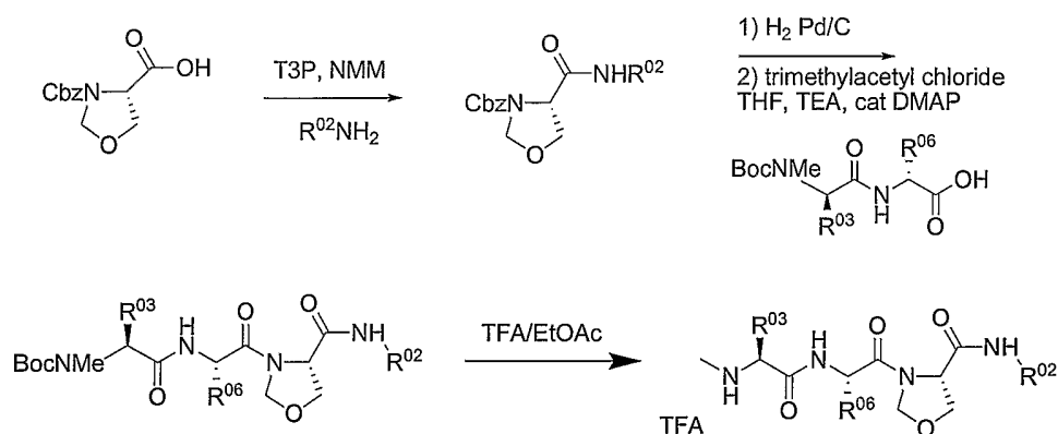
Scheme 14:
