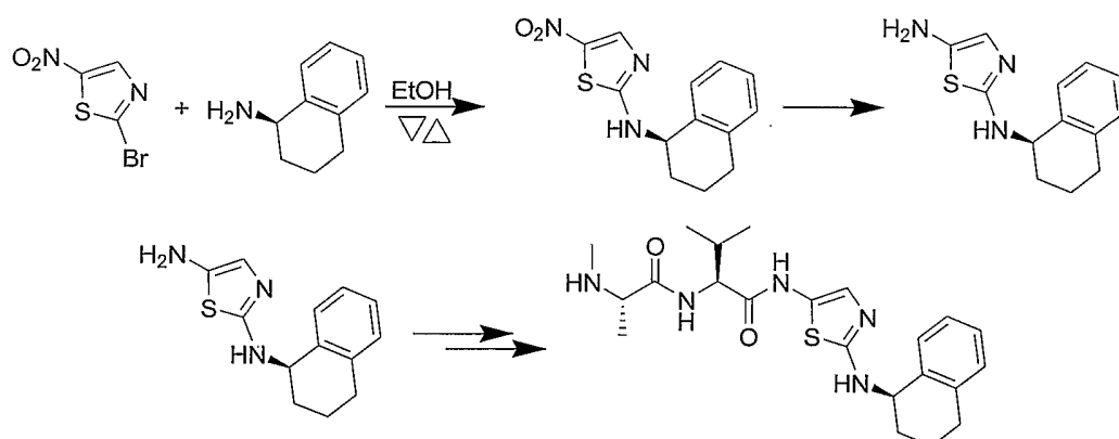
Scheme 29:
