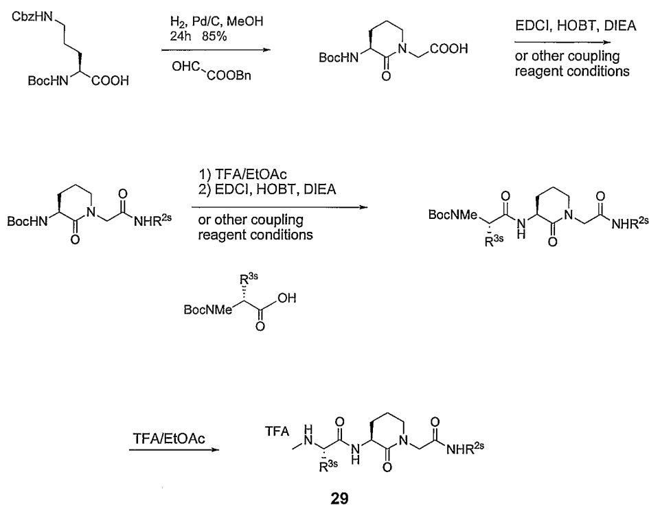
Scheme 10
