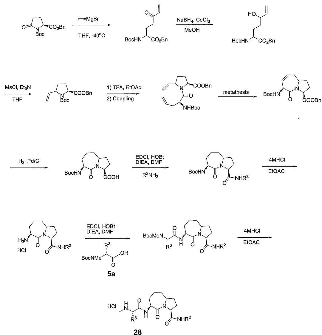
Scheme 9
