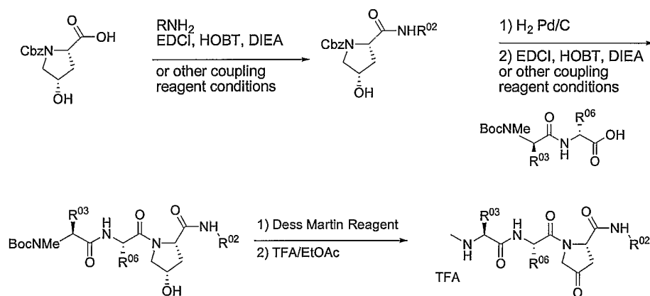
Scheme 16:
