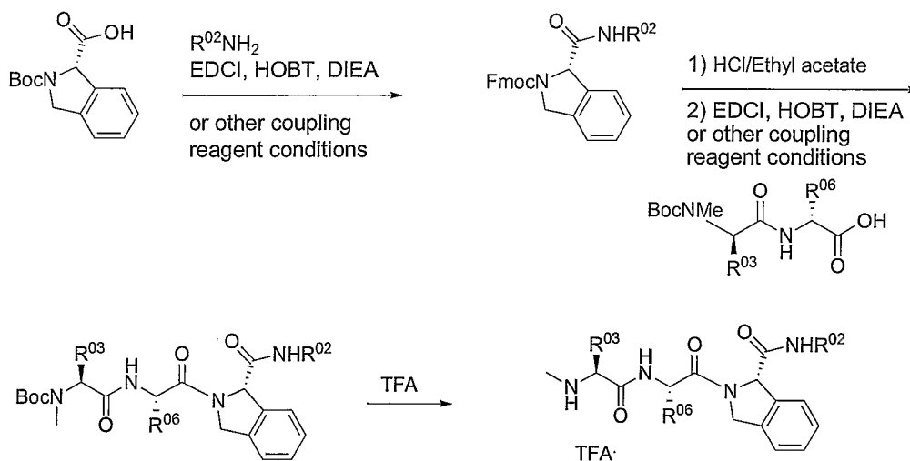
Scheme 20:
