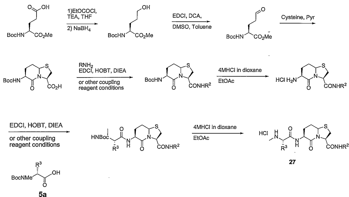
Scheme 8
