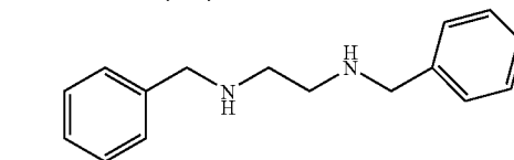
N,N'-dibenzylethylene diamine
