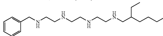
N-benzyl-N'''-(2-ethylhexyl)triethylene tetramine
