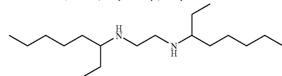
N,N'-bis(2-ethylhexyl)ethylenediamine
