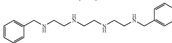
N,N'''-dibenzyltriethylene tetramine
