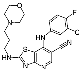
Cpd. No. 8
