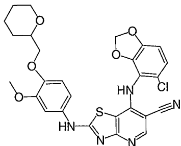
Cpd. No. 43
