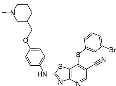
Cpd. No. 40
