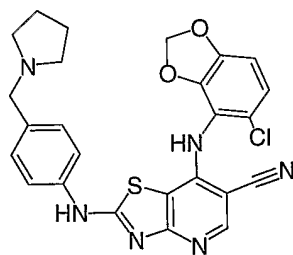
Cpd. No. 45
