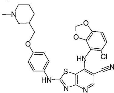
Cpd. No. 40
