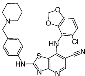
Cpd. No. 41
