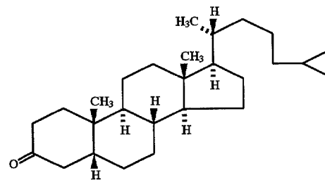
5 \beta -Cholestan-3-one
