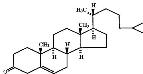
5-Cholesten-3-one
