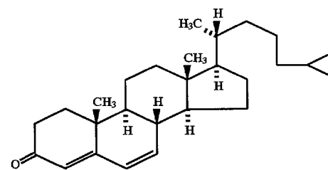
Cholesta-4,6-dien-3-one
