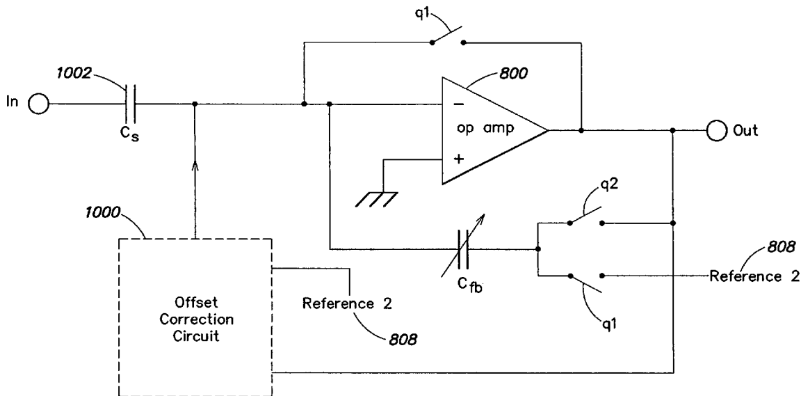
CDS/PxGA Circuit with Offset Correction
