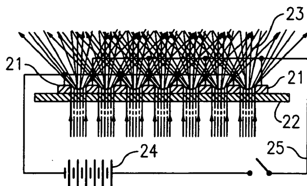
FIG. 6 Prior Art
