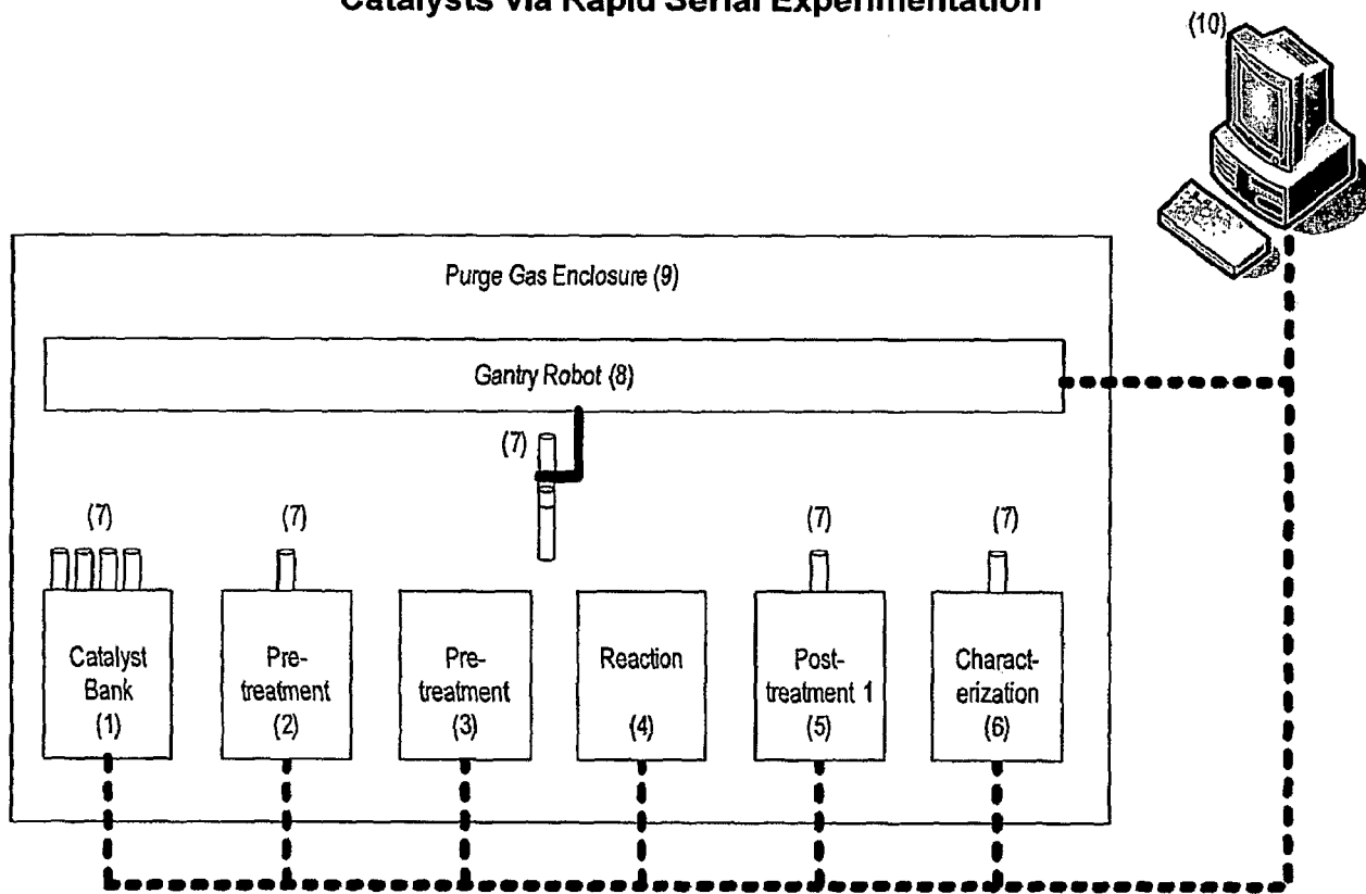
Exemplary Schematic of Process for Testing Catalysts via Rapid Serial Experimentation
