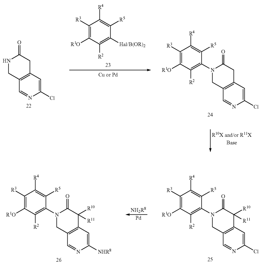
Scheme 5
