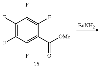
Scheme 3
