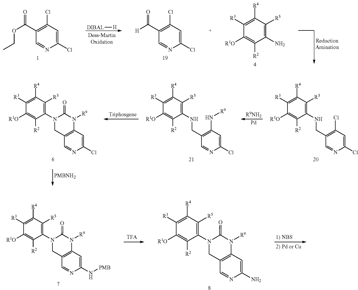
Scheme 4
