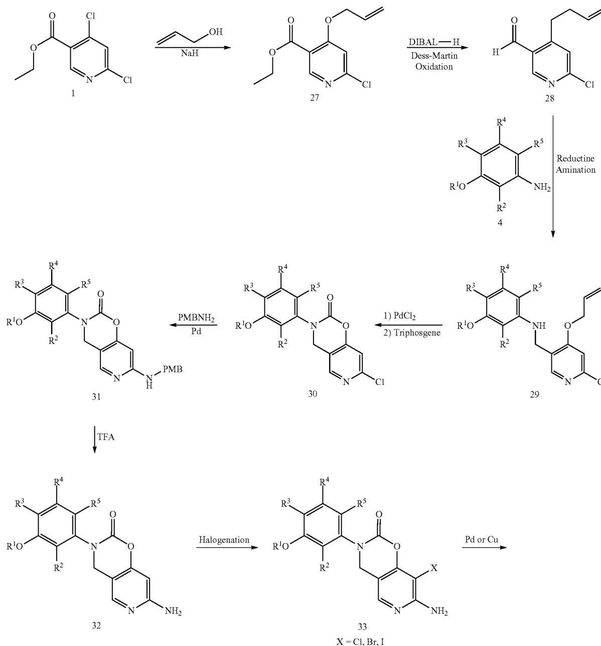
Scheme 6
