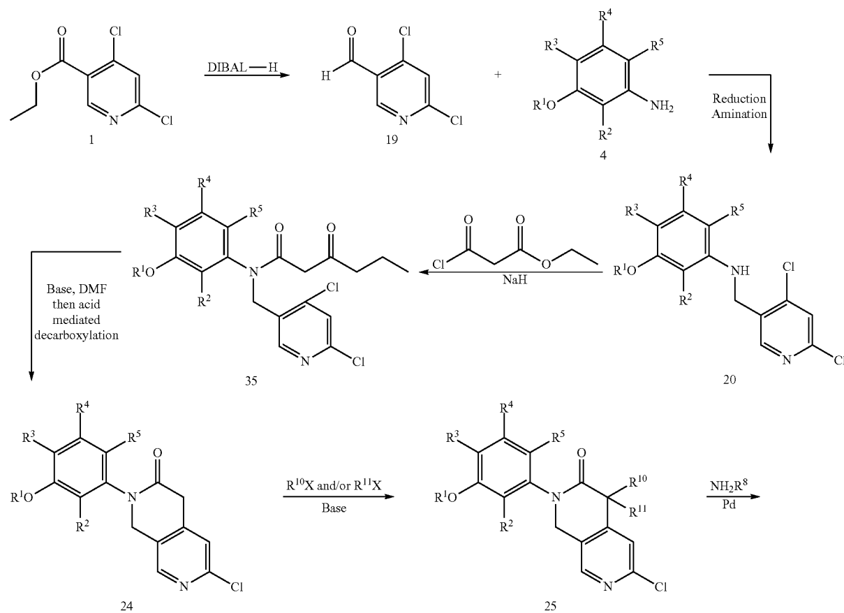
Scheme 7
