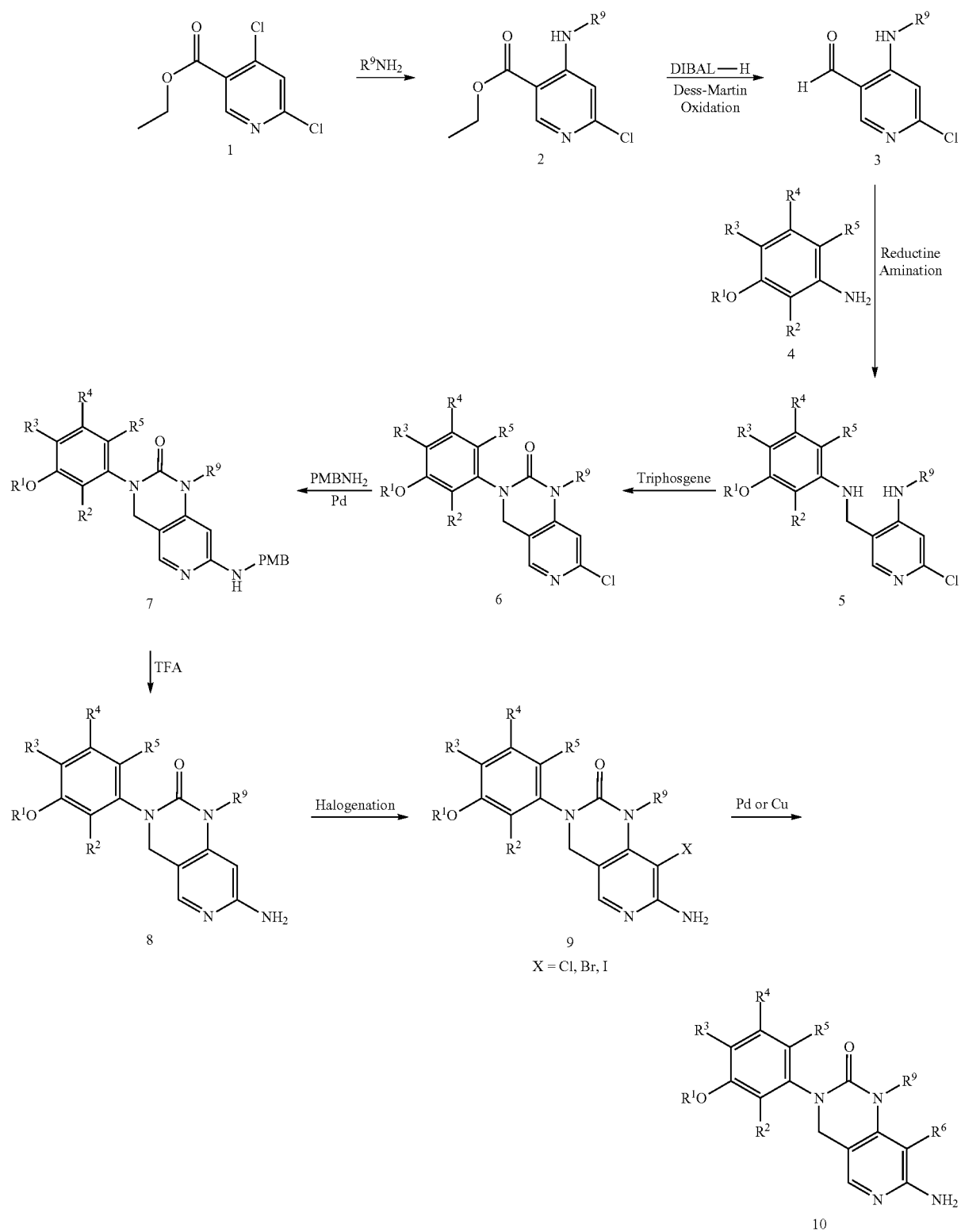
Scheme 1
