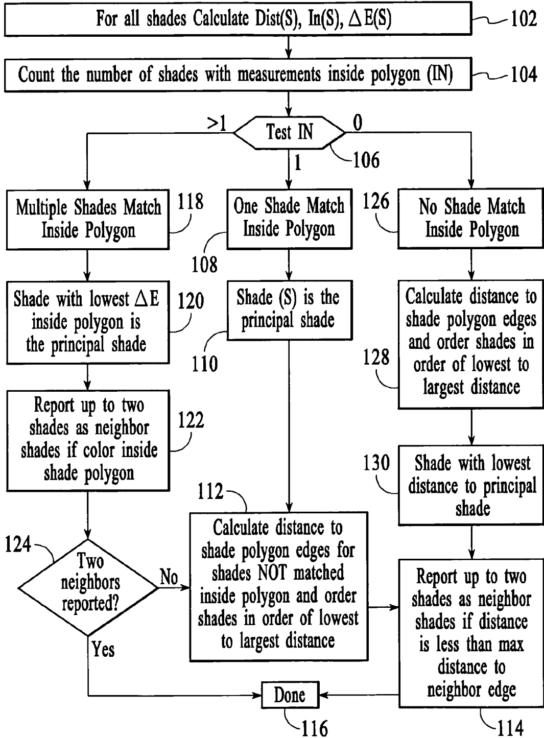
LCH Shade matching
