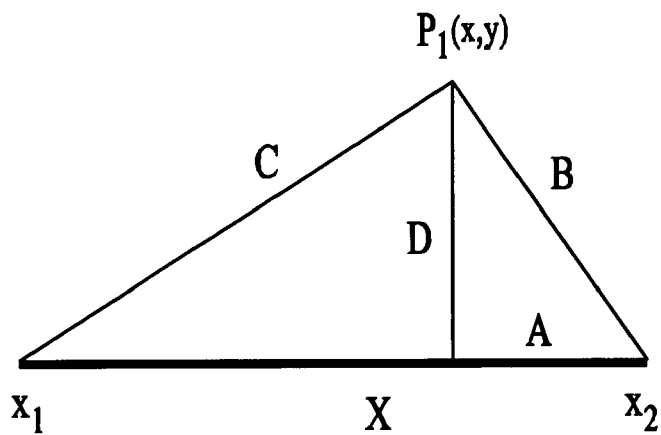
Shortest distance to a line segment
