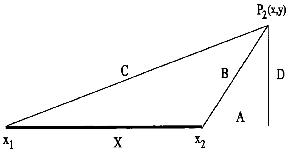
Shortest distance to a line segment
