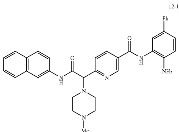
N-(4-aminobiphenyl-3-yl)-6-[1-(4-methylpiperazin-1-yl)-2-(2-naphthylamino)-2-oxoethyl]nicotinamide. The
