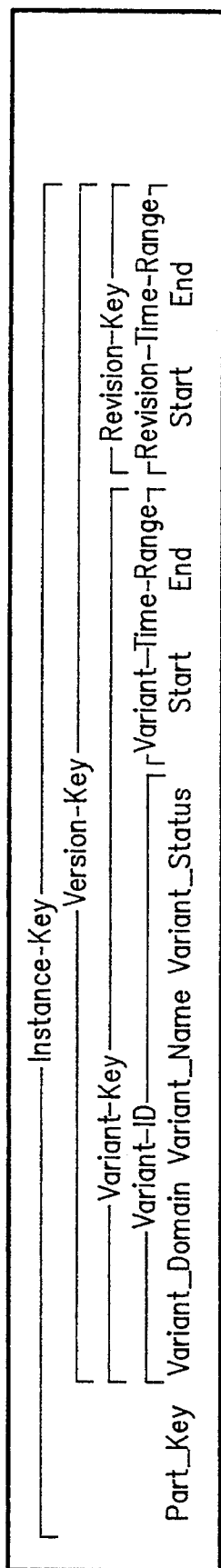
COMPONENTS OF AN ENTITY INSTANCE KEY
