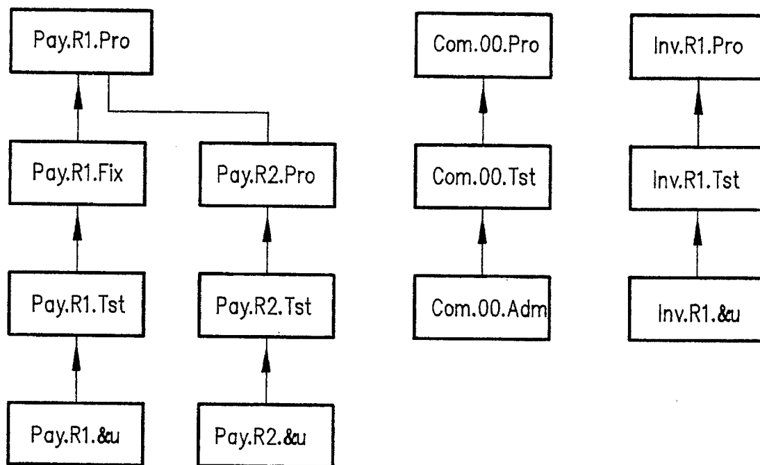
VARIANT HIERARCHIES FOR THE PAY, COM, AND INV VARIANT DOMAINS
