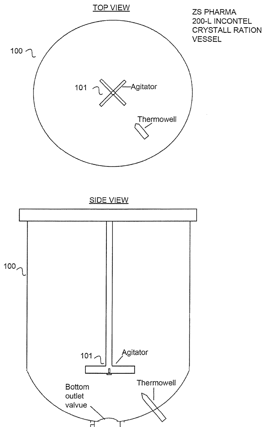
Fig. 17: 200-L reaction vessel with standard agitator arrangement.
