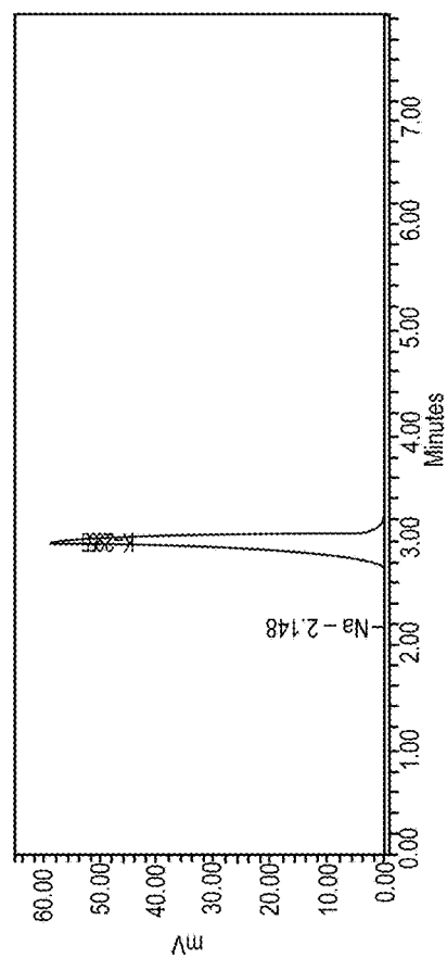
Fig. 15: Example of the Assay Standard Solution Chromatogram.
