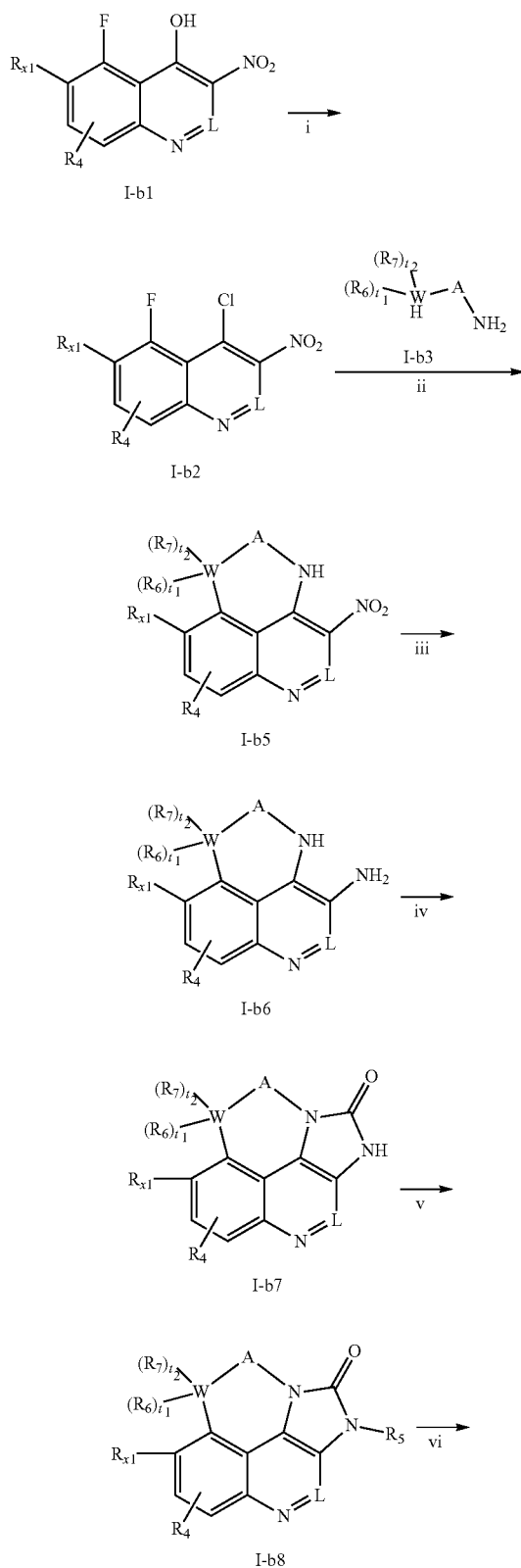
synthetic scheme 3:
