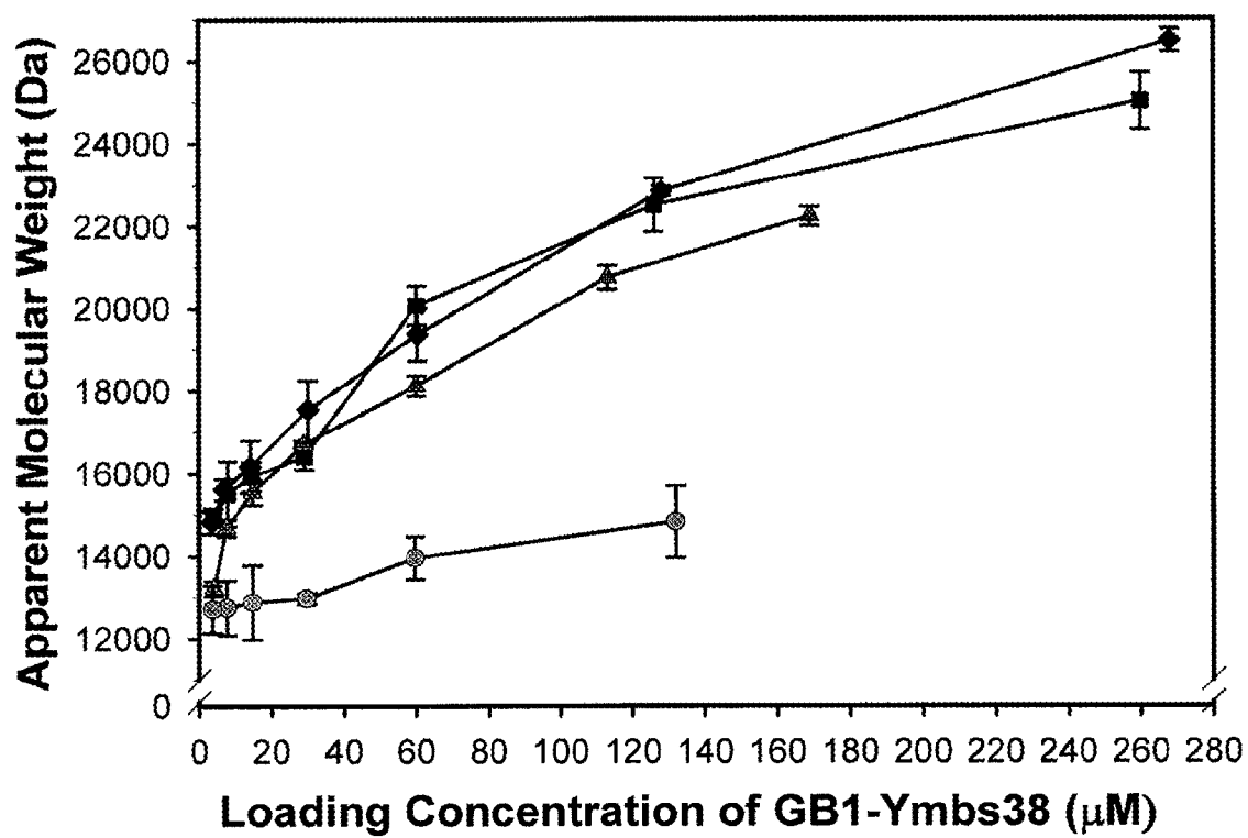
Figure 23. Comparison of Large Zone Chromatography Assays on GB1-Ymbs38
