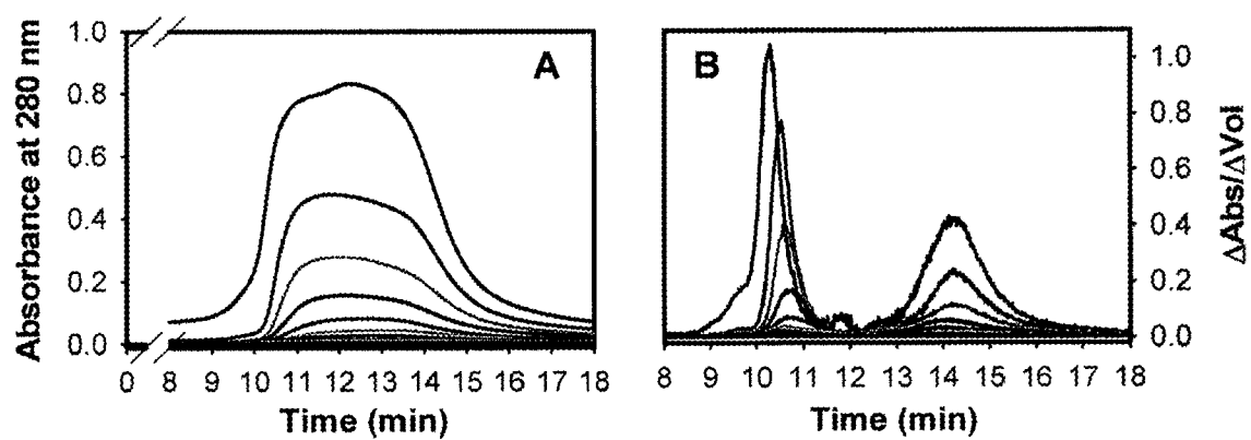
Figure 22. Large Zone Size Exclusion Chromatography on Zn(II)CopY
