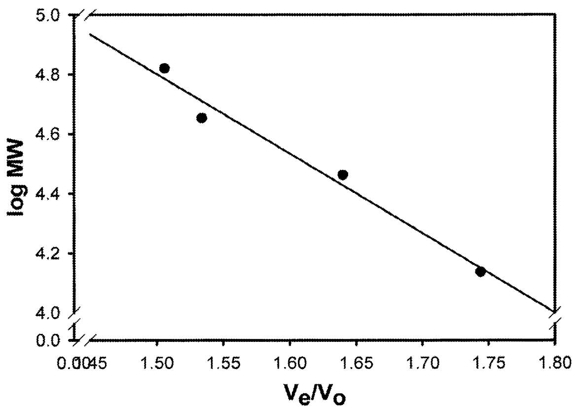
Figure 11. Molecular weight standard curve for the Shodex KW 803 HPLC column
