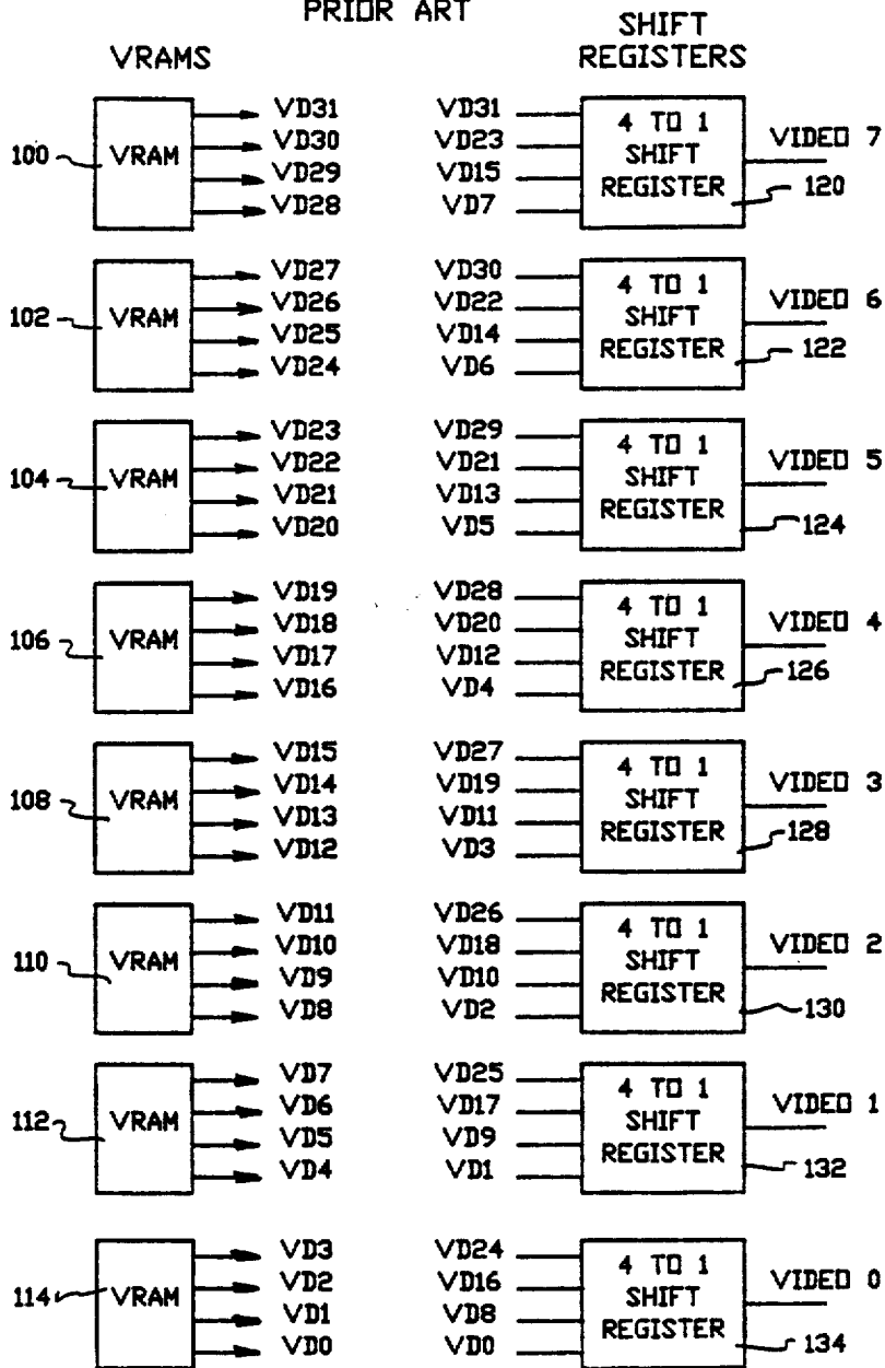
FIG.1 PRIOR ART
