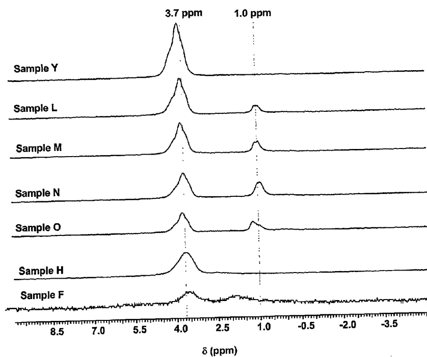
Figure 3. MAS ^1\text{H} NMR of modified SAPO-34 via different methods
