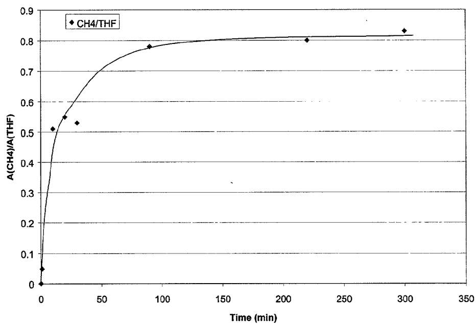
Figure 2. Evolution of methane during MeMgBr treatment of SAPO-34 in toluene/THF (Example 18)
