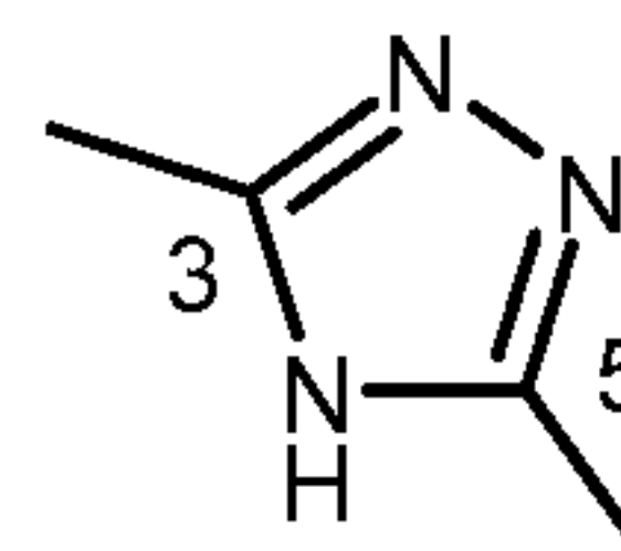
4H-tautomer
