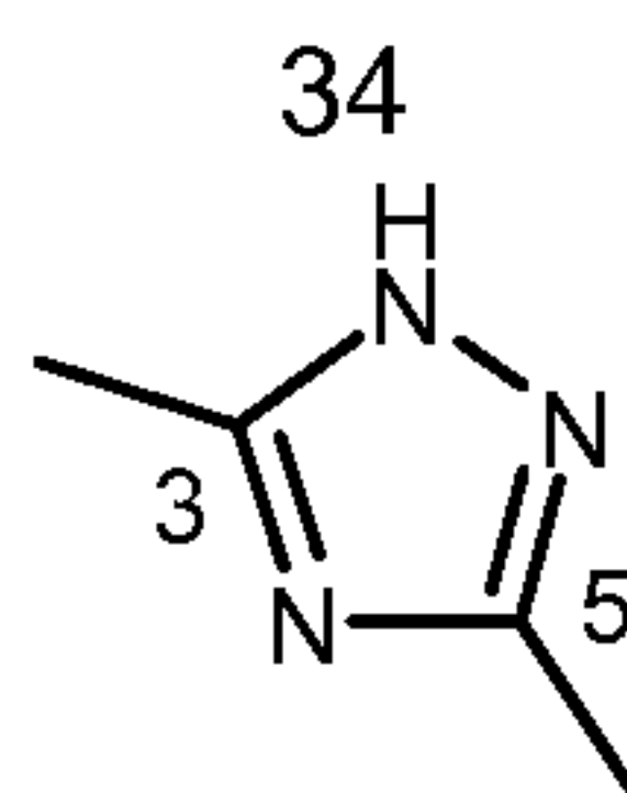
2H-tautomer
