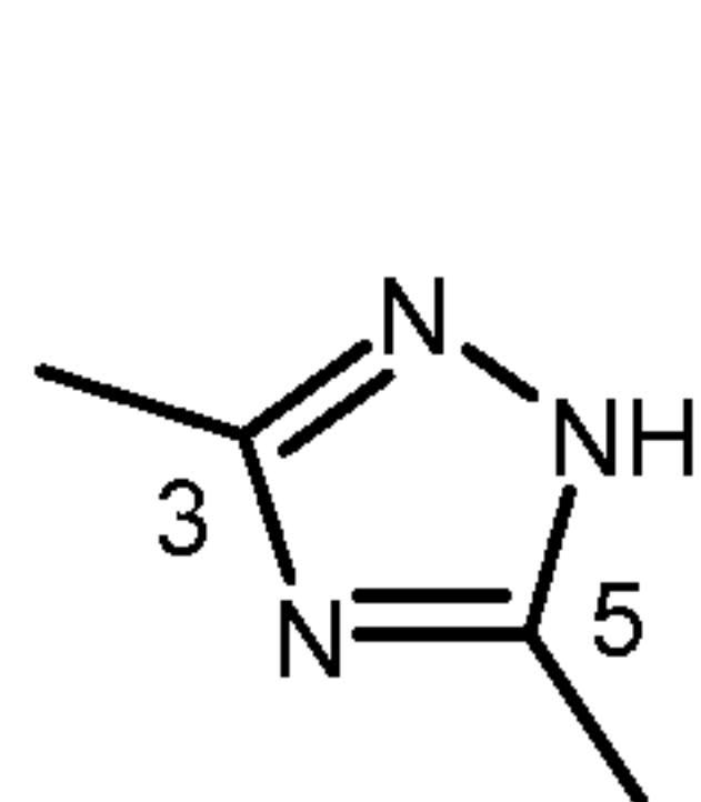
1H-tautomer
