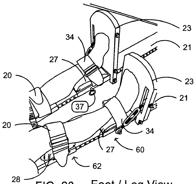
FIG. 20 Foot / Leg View
