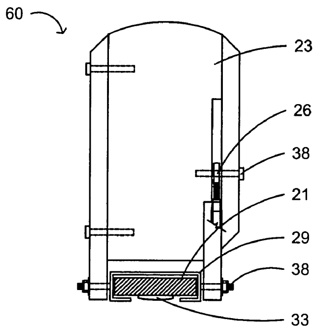
Foot Paddle - Front View
