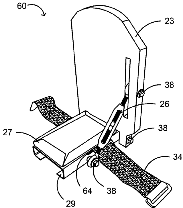
FIG. 10 Sliding Foot Mechanism
