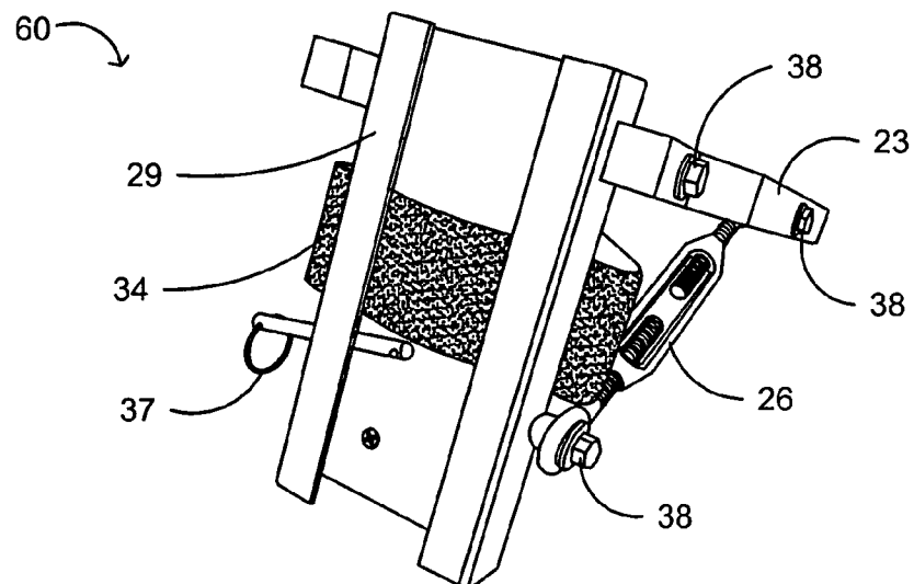
FIG. 11 Bottom View
