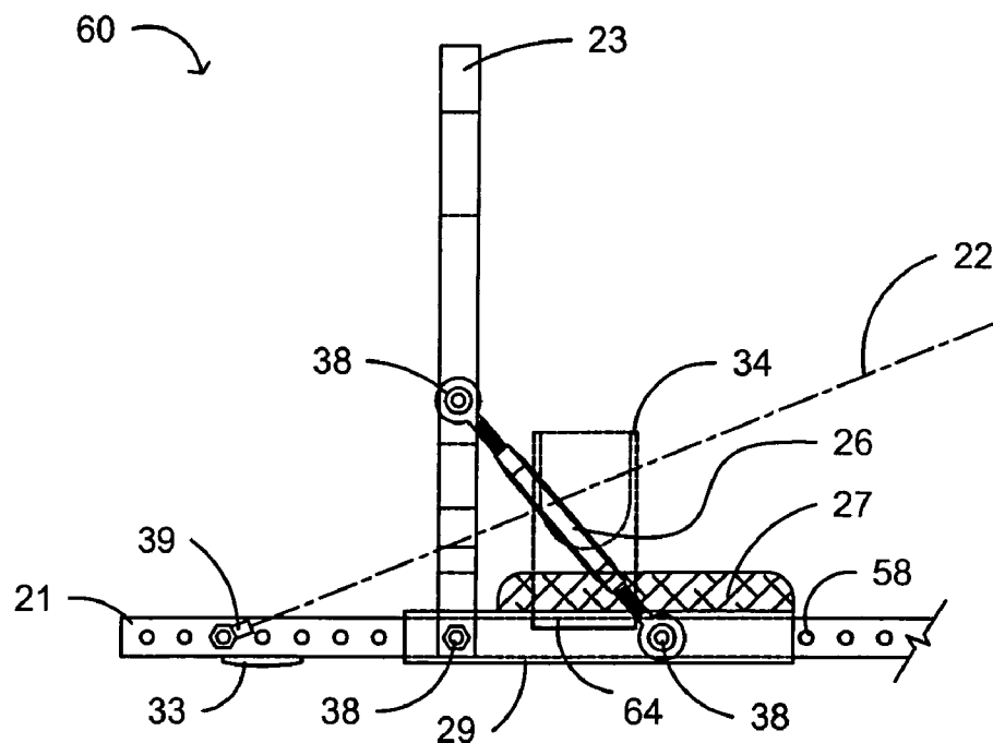
Foot Paddle - Side View
