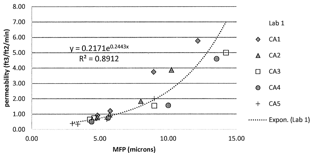
Permeability vs MFP: Method 1, Lab 1
