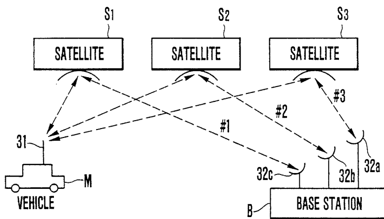
FIG. 1 (PRIOR ART)
