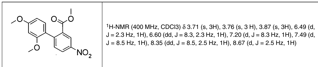
3-Hydroxy-8-nitrobenzo[c]chromen-6-one (Reference Compound No.1-1-(2))
