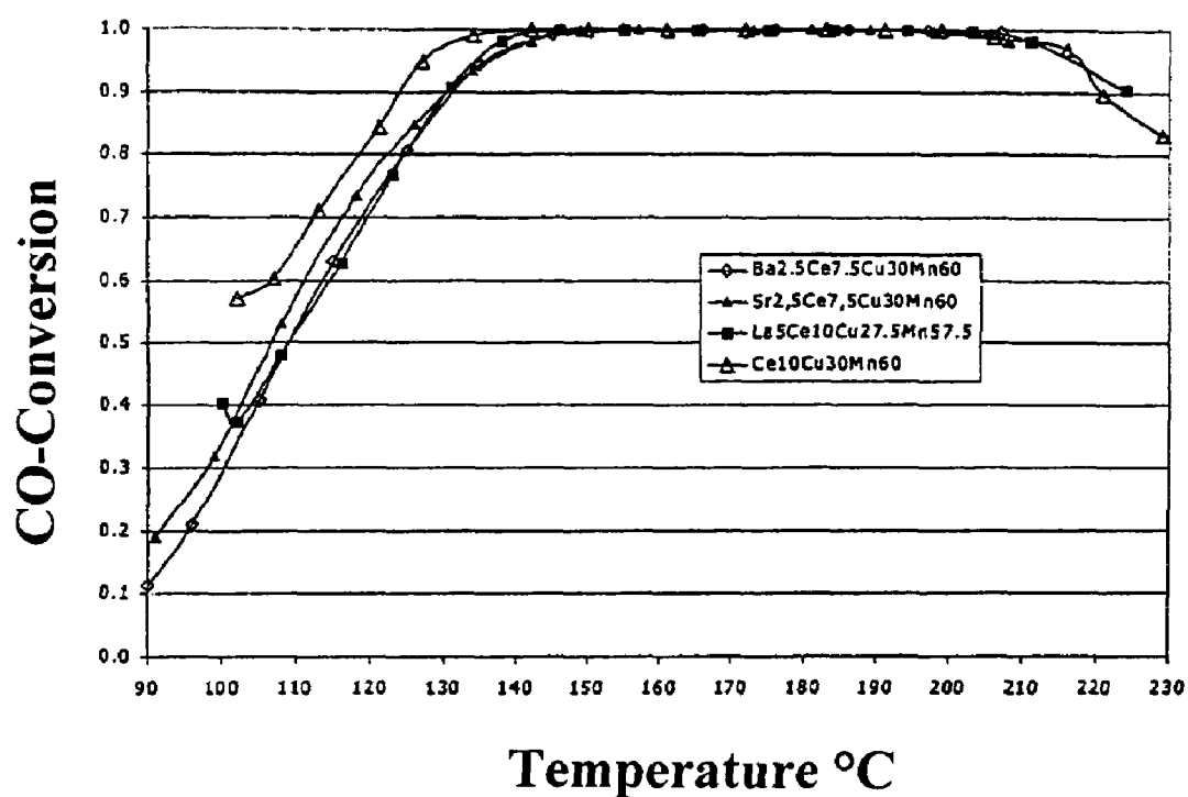
Fig. 7: The activity in CO-oxidation of various catalysts in dependency of the temperature.
