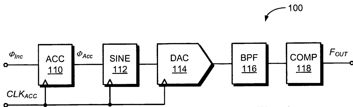
Fig. 1 (Prior Art)
