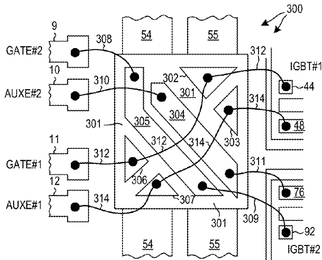
BRIDGING DMB STRUCTURE (TOP VIEW)
