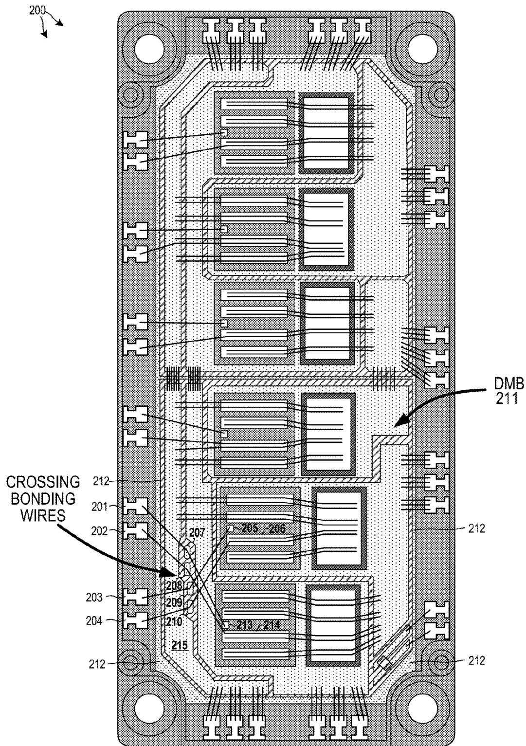
POWER SEMICONDUCTOR DEVICE MODULE (Prior Art)
