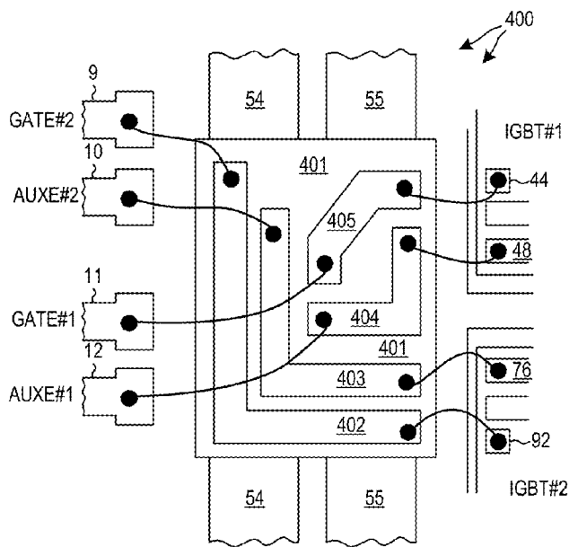
BRIDGING DMB STRUCTURE (TOP VIEW)
