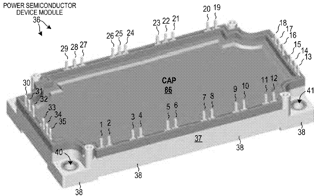
POWER SEMICONDUCTOR DEVICE MODULE
