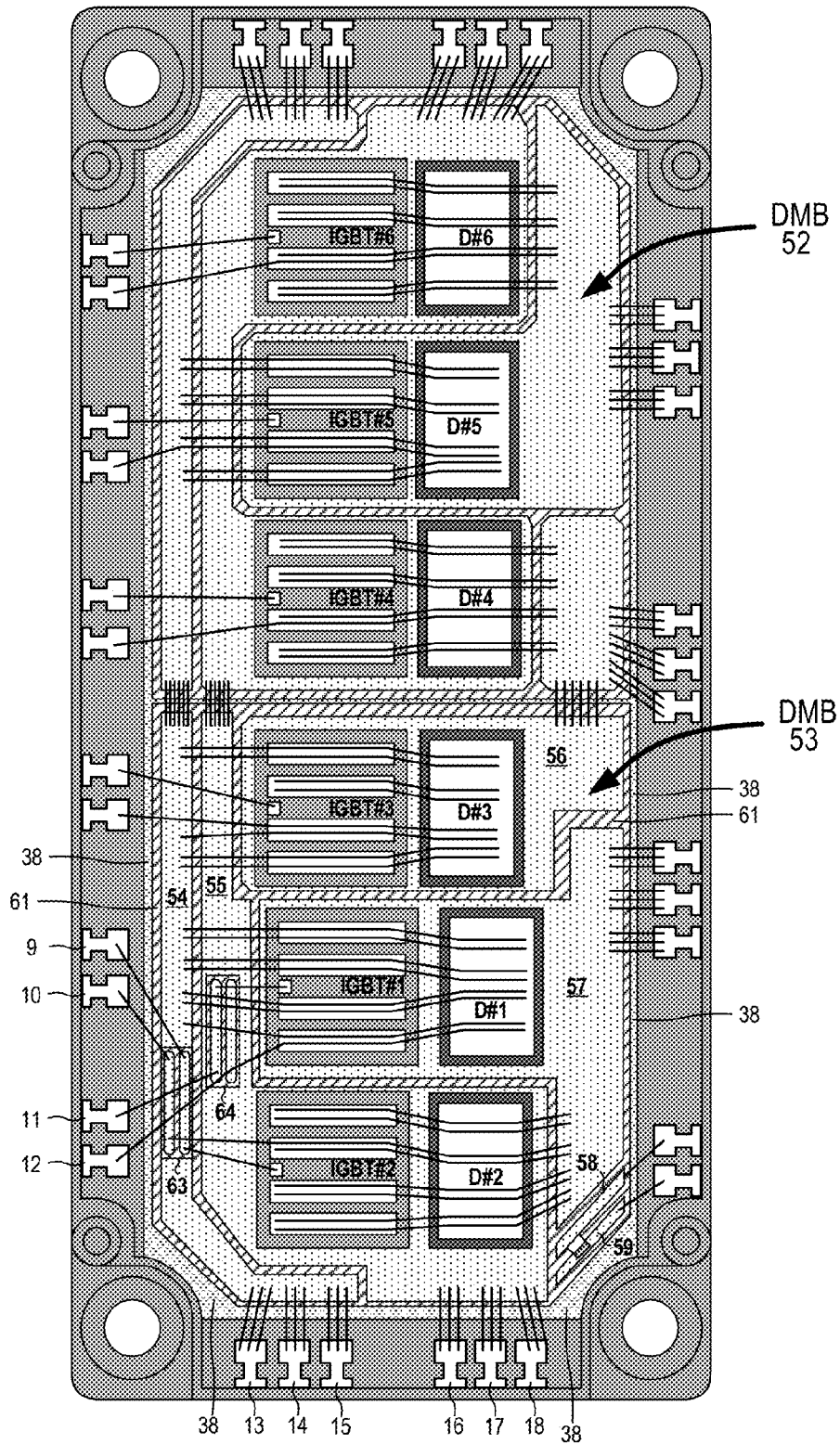
POWER SEMICONDUCTOR DEVICE MODULE
