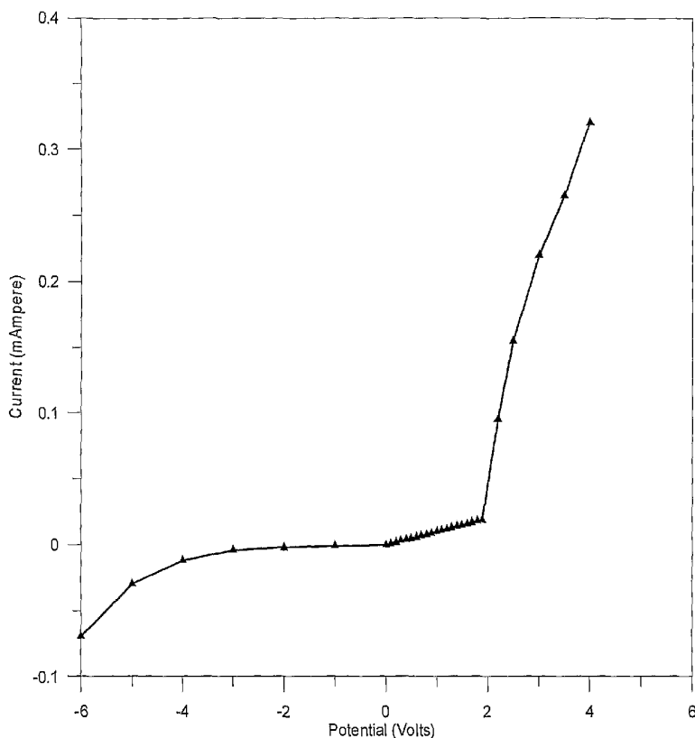
Current - Voltage Plot of a Zinc Oxide P/N Junction
