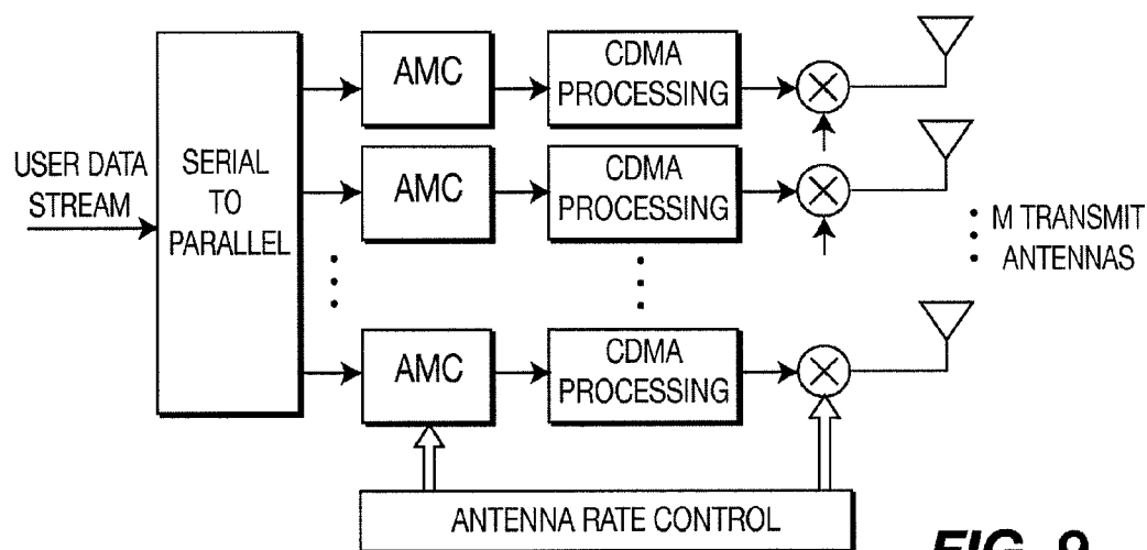
FIG. 9 PRIOR ART
