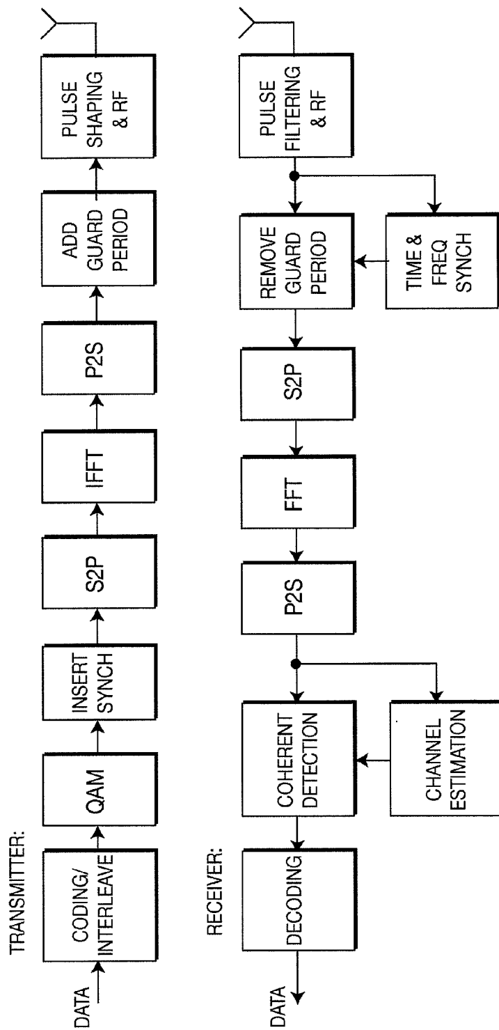
FIG. 3 PRIOR ART
