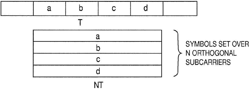
FIG. 2 PRIOR ART
