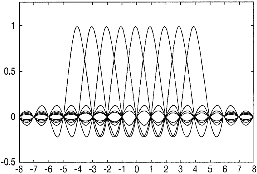
FIG. 1 PRIOR ART
