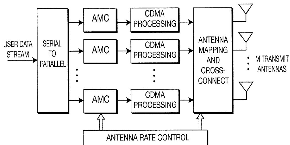
FIG. 10 PRIOR ART
