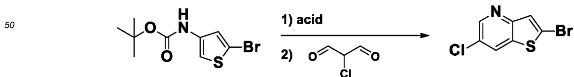
Scheme 3
