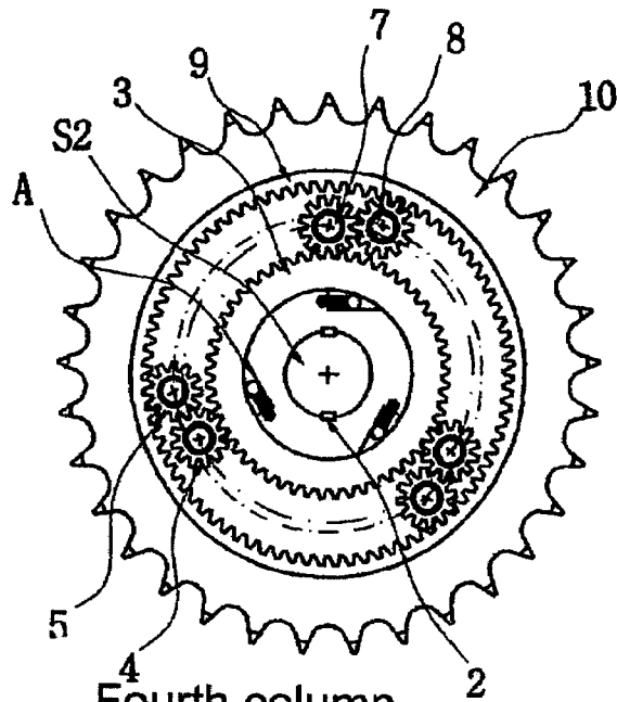
Fourth column Cross section of a group of clockwise one-way clutche
