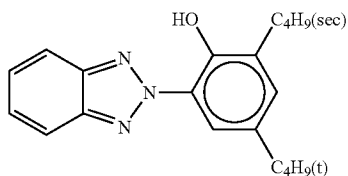
(UV-5) ULTRAVIOLET RAY ABSORBENT
